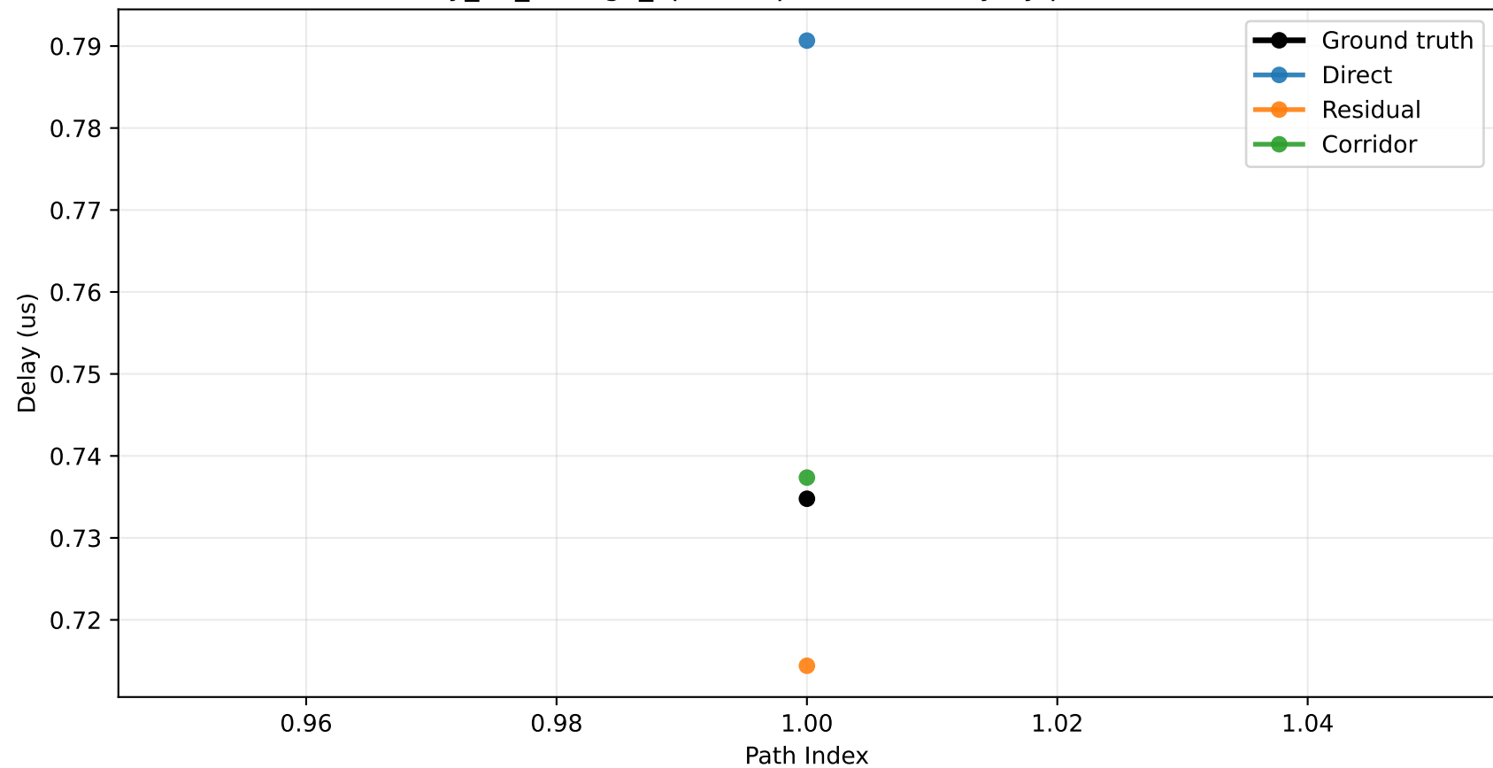
city_47_chicago_3p5 sample 1500: delay by path index
