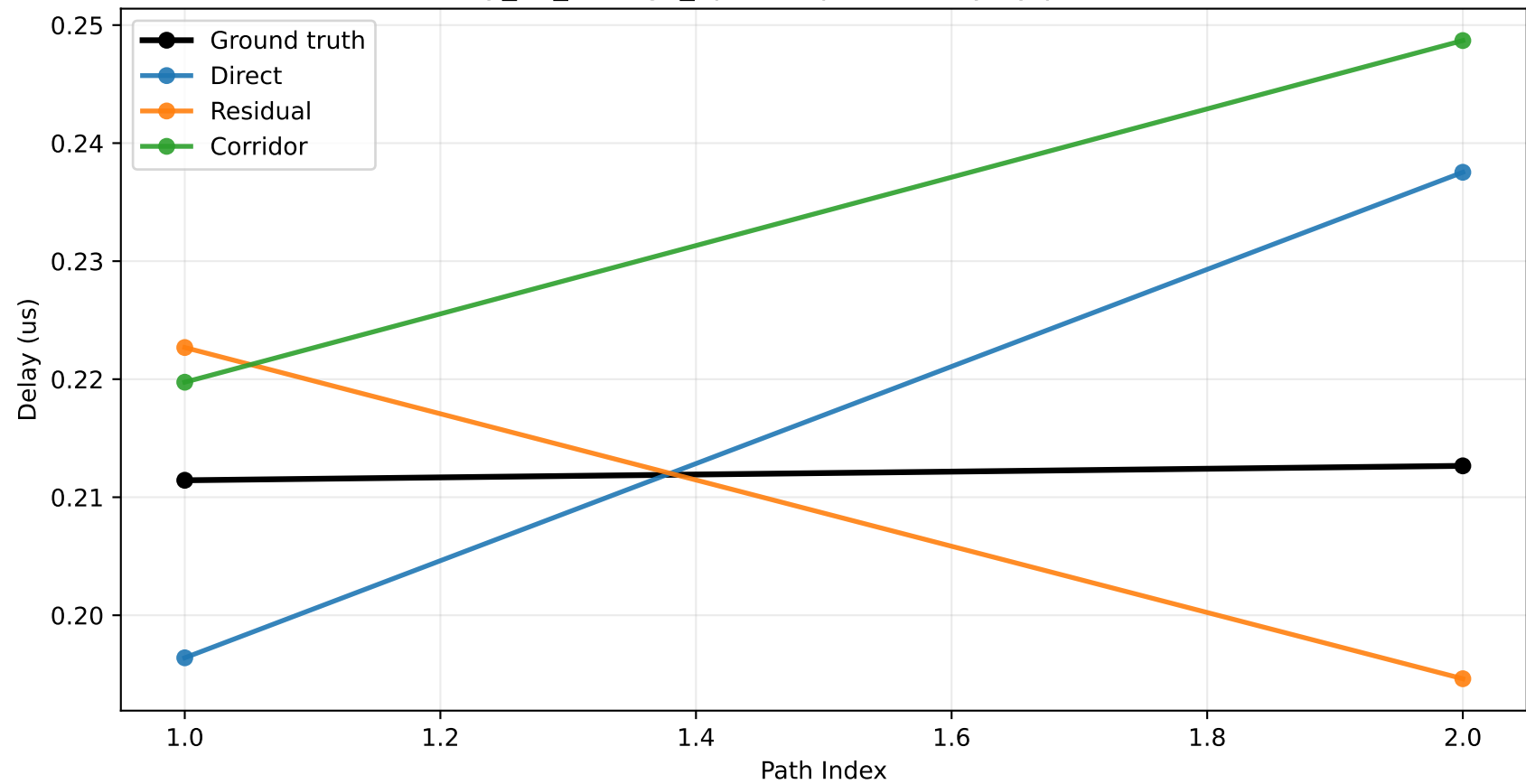
city_47_chicago_3p5 sample 5: delay by path index
