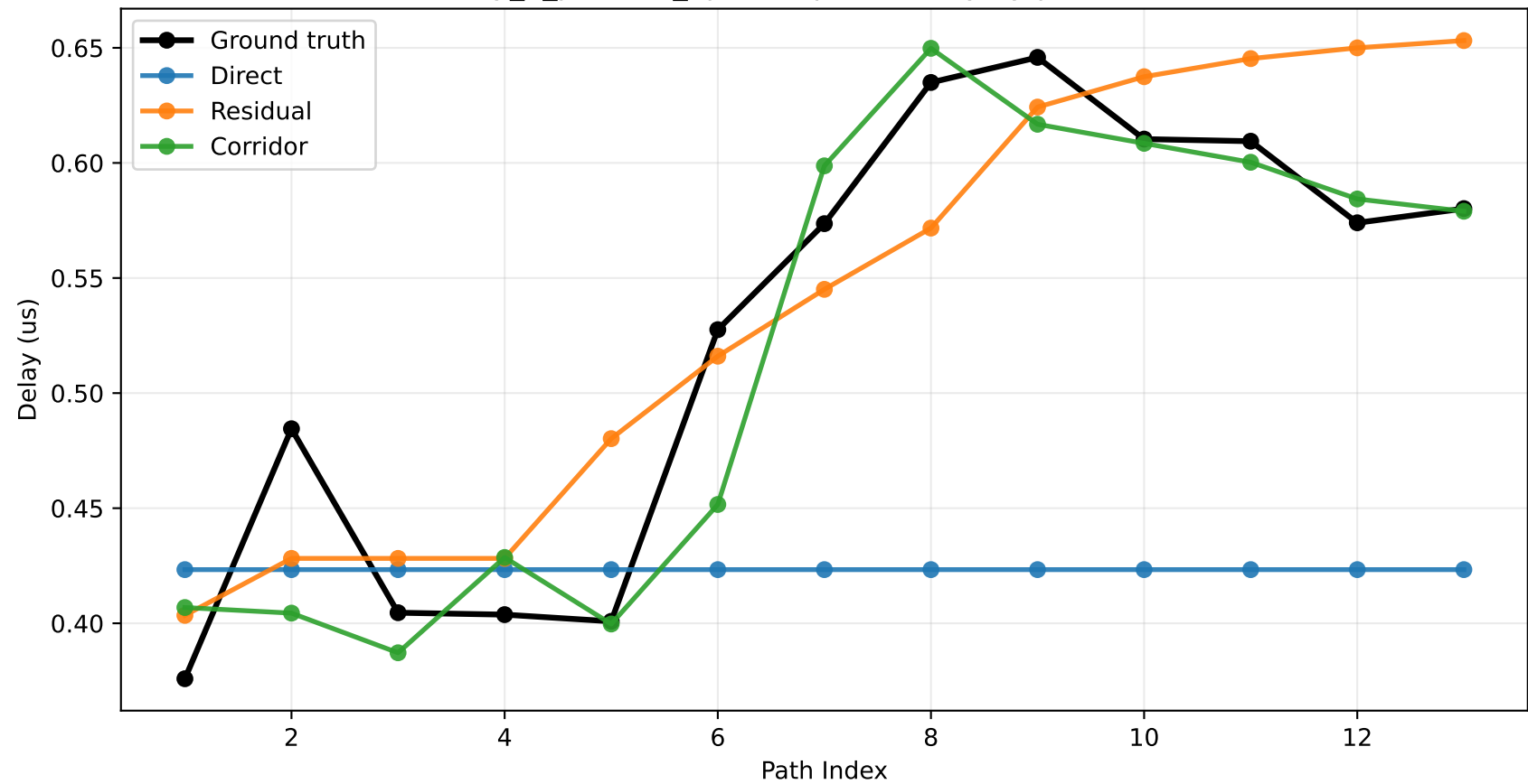
city_4_phoenix_3p5 sample 0: delay by path index
