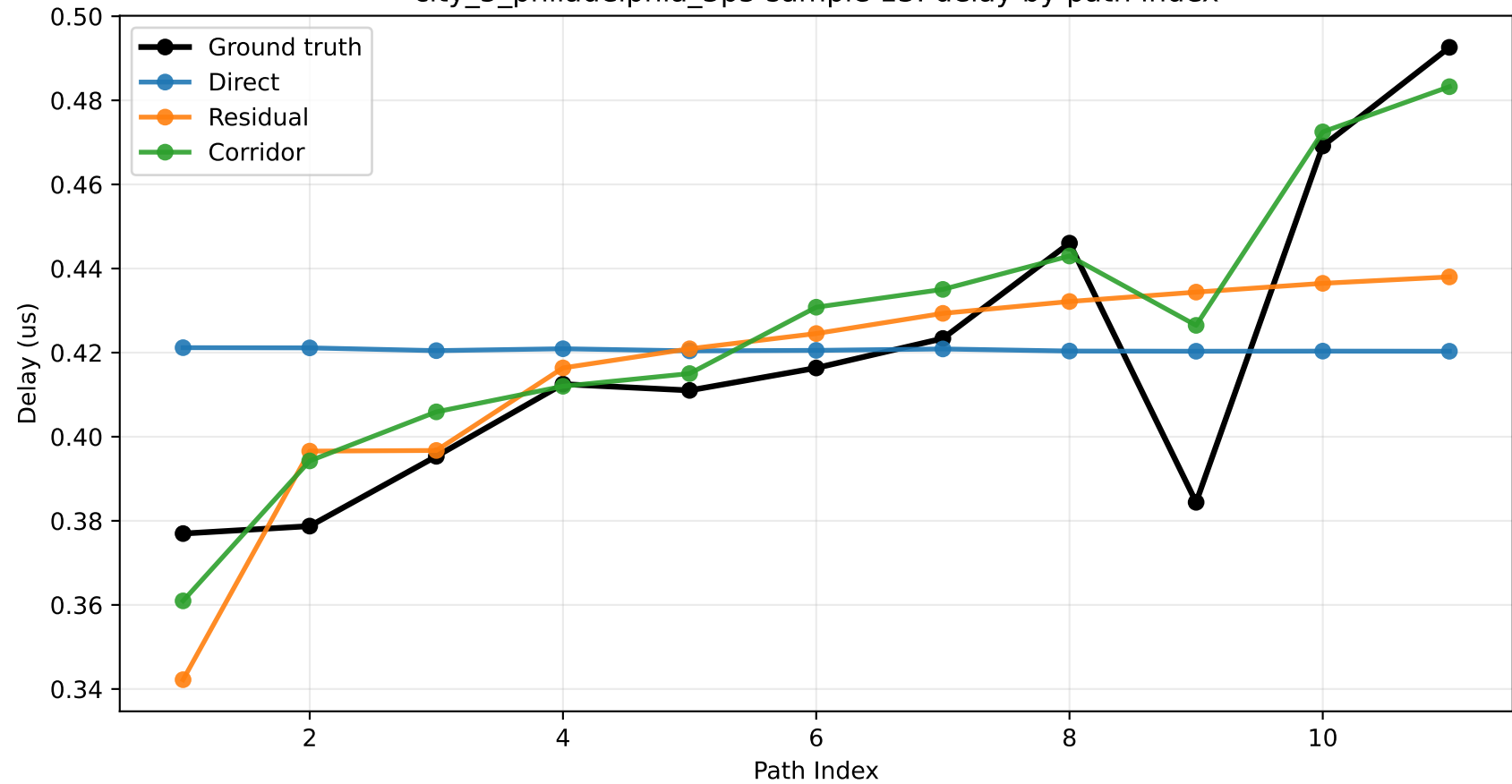
city_5_philadelphia_3p5 sample 13: delay by path index
