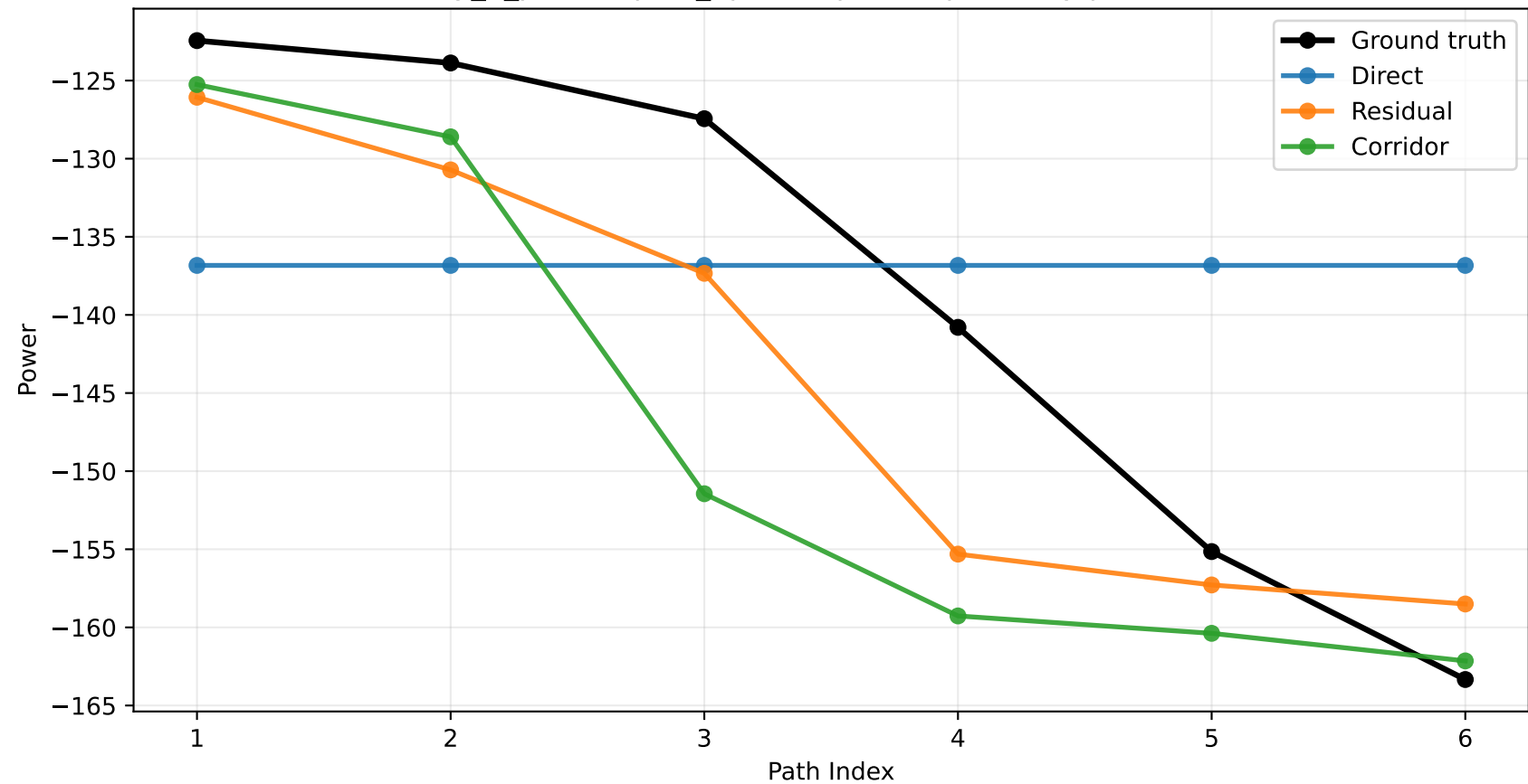
city_5_philadelphia_3p5 sample 21: power by path index
