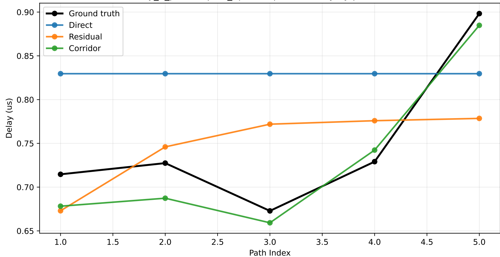
city_5_philadelphia_3p5 sample 25: delay by path index
