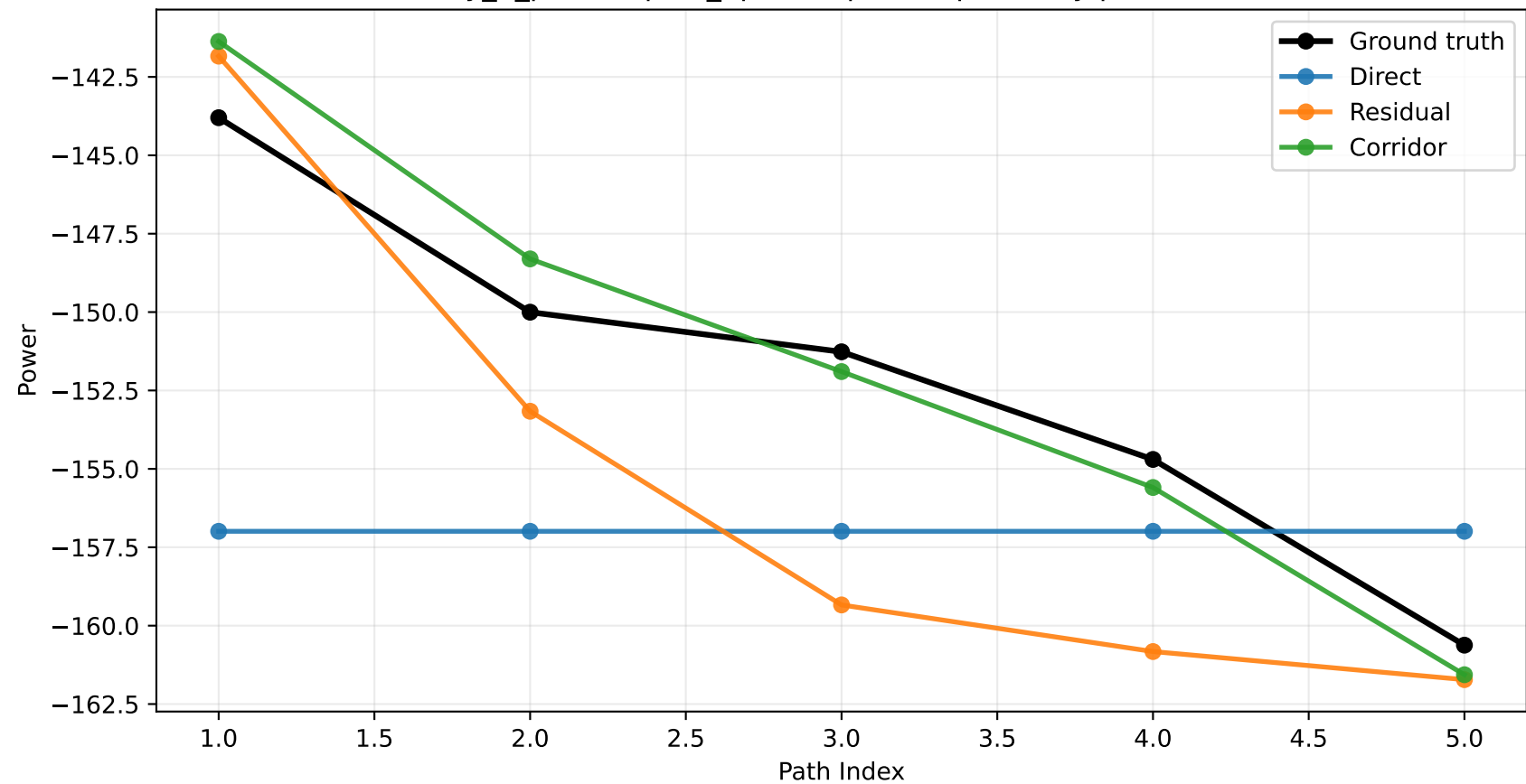
city_5_philadelphia_3p5 sample 25: power by path index
