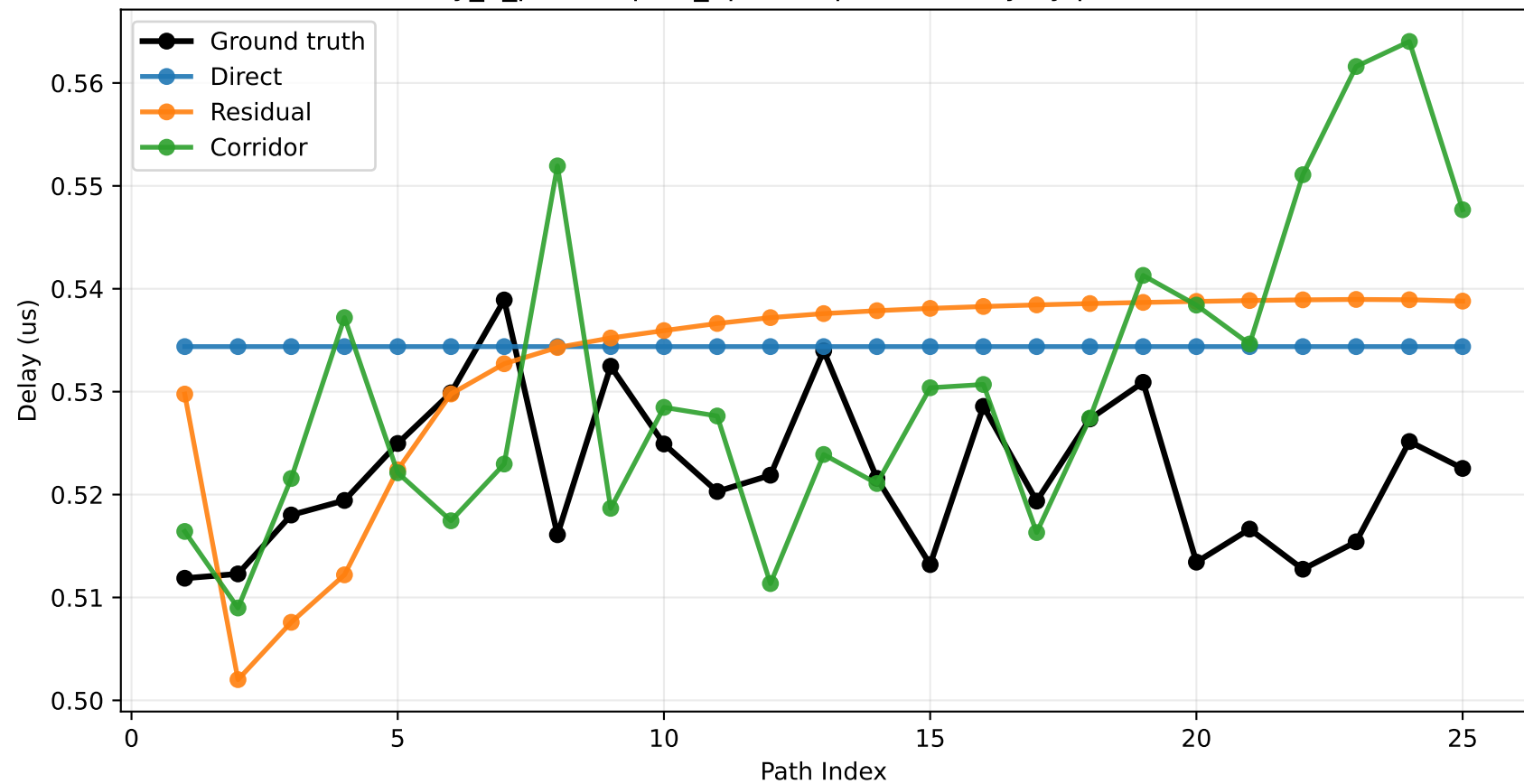
city_5_philadelphia_3p5 sample 55: delay by path index
