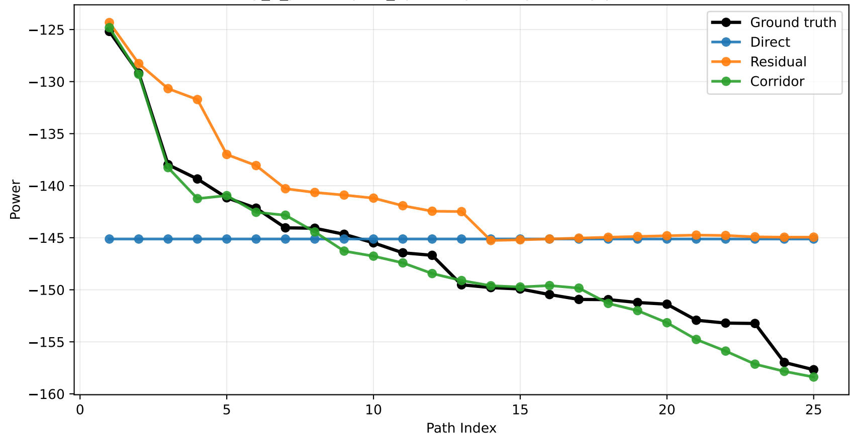
city_5_philadelphia_3p5 sample 65: power by path index
