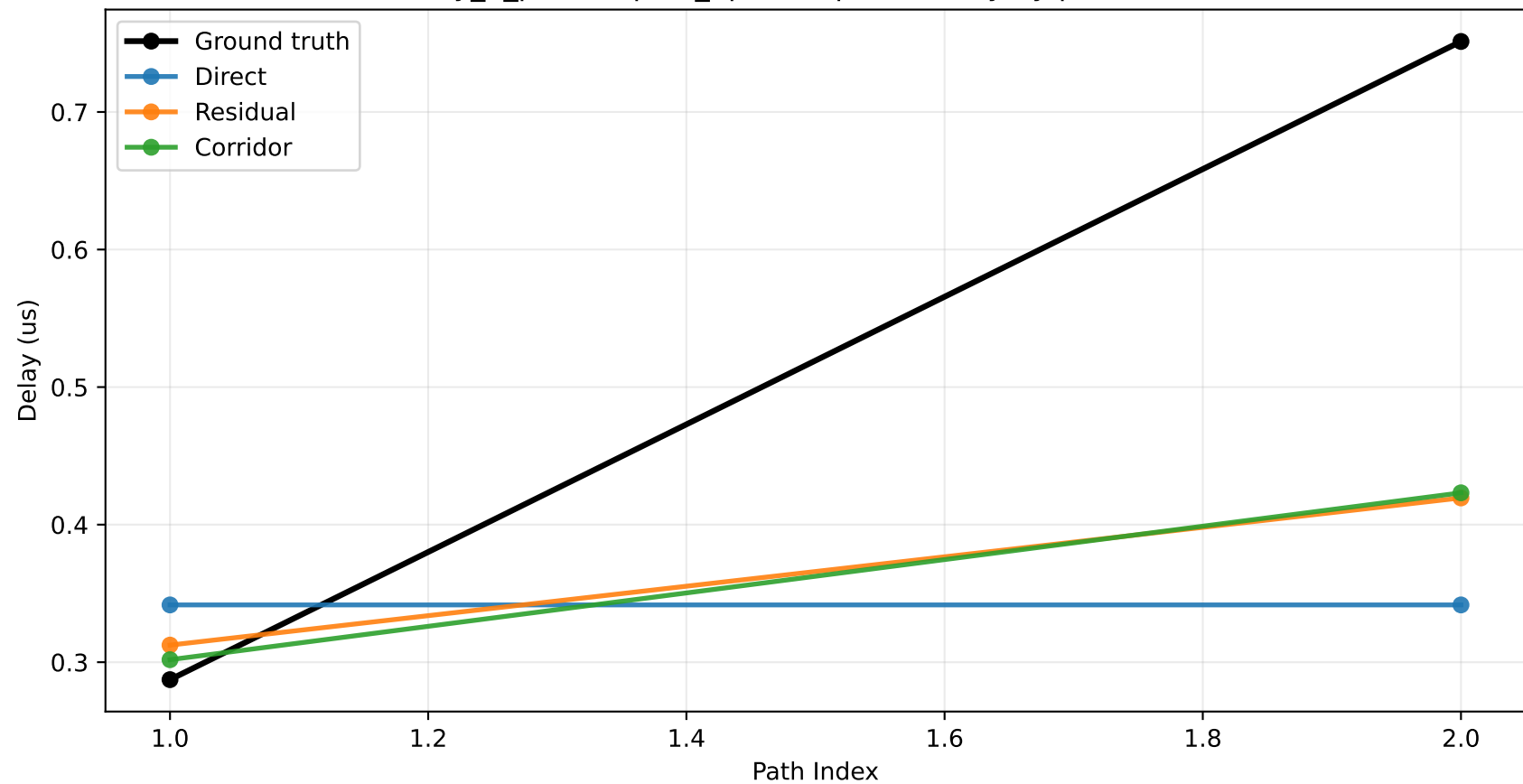
city_5_philadelphia_3p5 sample 8: delay by path index
