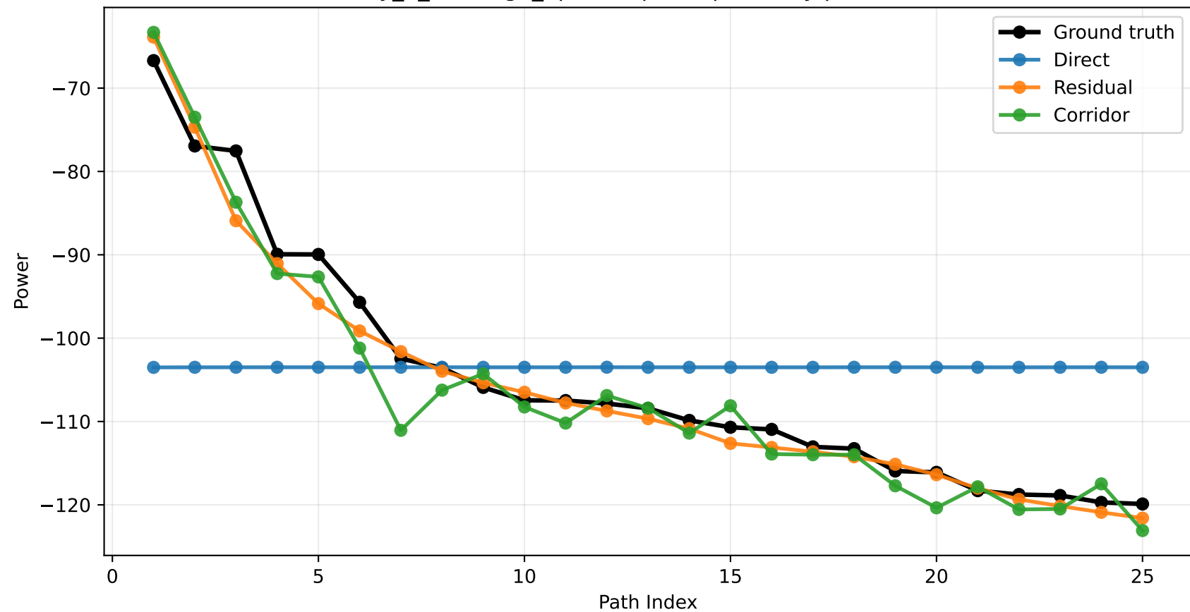
city_7_sandiego_3p5 sample 0: power by path index
