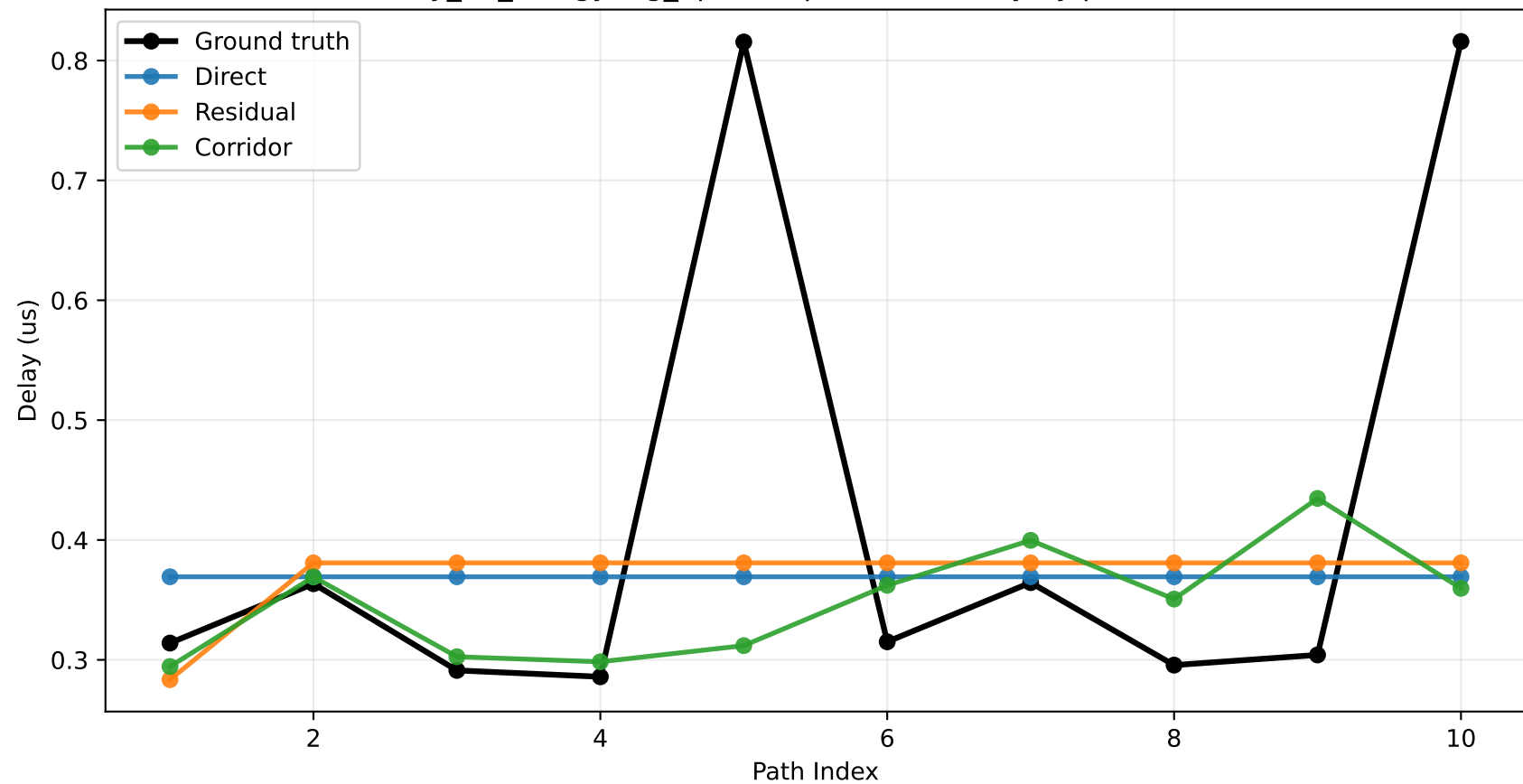
city_91_xiangyang_3p5 sample 1500: delay by path index
