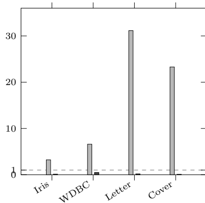
(c) EDP
