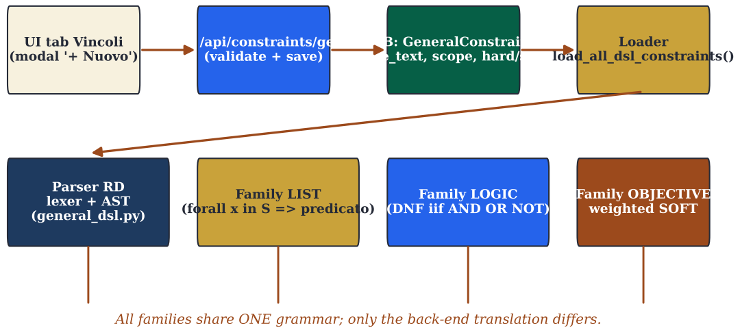
FIGURE 10.3 – Architecture of the general DSL: the same grammar and AST, four translation back-ends. Evaluating a solution (post-hoc evaluator) and building a model (compiler to CP-SAT) are two different traversals of the same tree.
