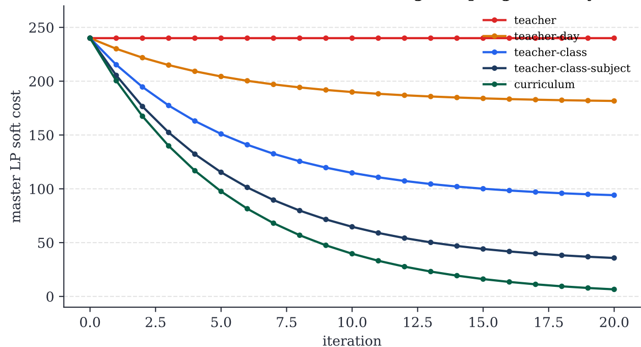
Branch-and-Price: master LP convergence per granularity
