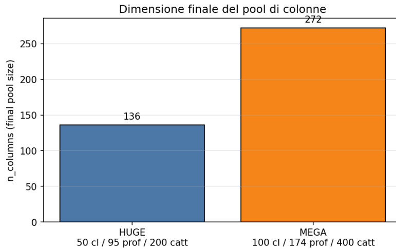
FIGURE 27.2 – Final column-pool size after the Branch-and-Price loop.
