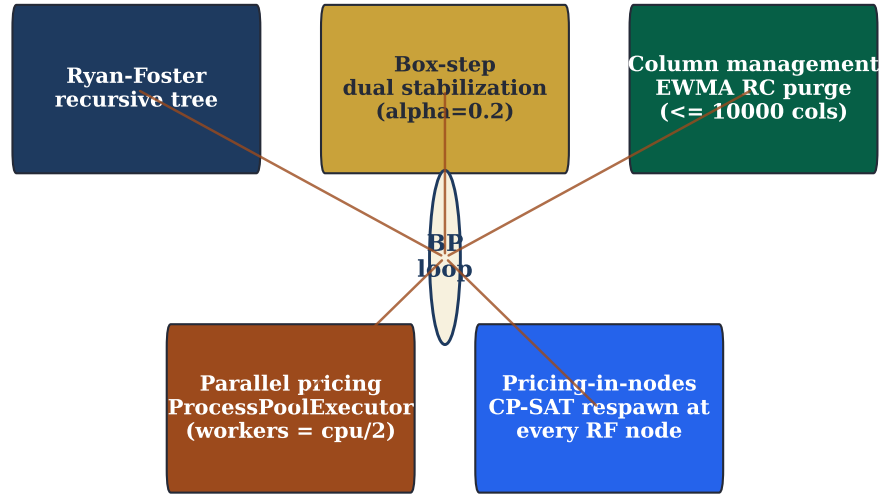
FIGURE 22.2 – Five composable scalability techniques around the Branch-and-Price loop: Ryan-Foster recursive tree, box-step dual stabilization, column management, parallel pricing, pricing-in-nodes (Step 4). All five are on by default in mode=”branch-and-price”.
