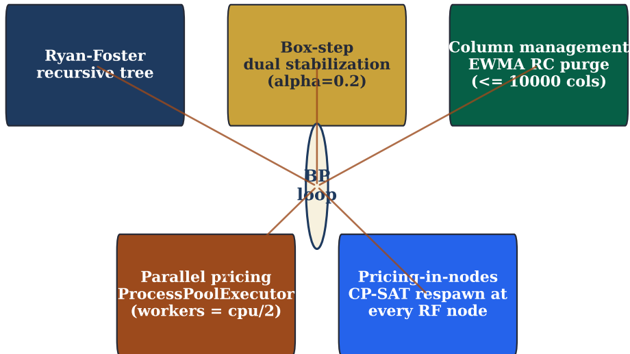
FIGURE 20.4 – Five composable scalability techniques around the Branch-and-Price loop: Ryan-Foster recursive tree, box-step dual stabilization, column management, parallel pricing, pricing-in-nodes (Step 4). All five are on by default in mode=”branch-and-price”.
