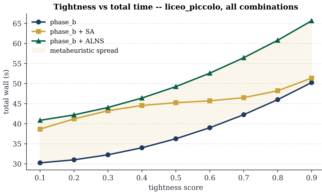
FIGURE 20.8 – Total time vs scenario tightness for the three dominant combinations (Phase B alone, + SA, + ALNS). The ivory band is the metaheuristic spread, growing with tightness.
