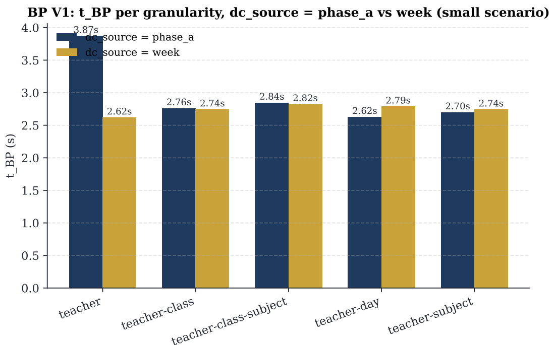
FIGURE 20.6 – Pricing time per granularity, with dc_source between Phase A (rigid) and weekly (cp_sat_scope=week). Small scenario shows no practical difference.
