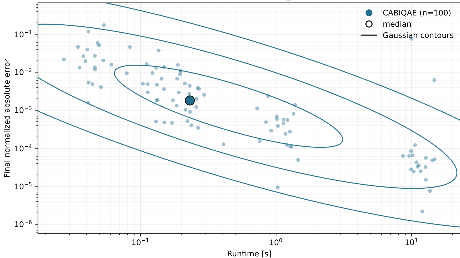
Final error versus runtime: ideal_v2 comparison
