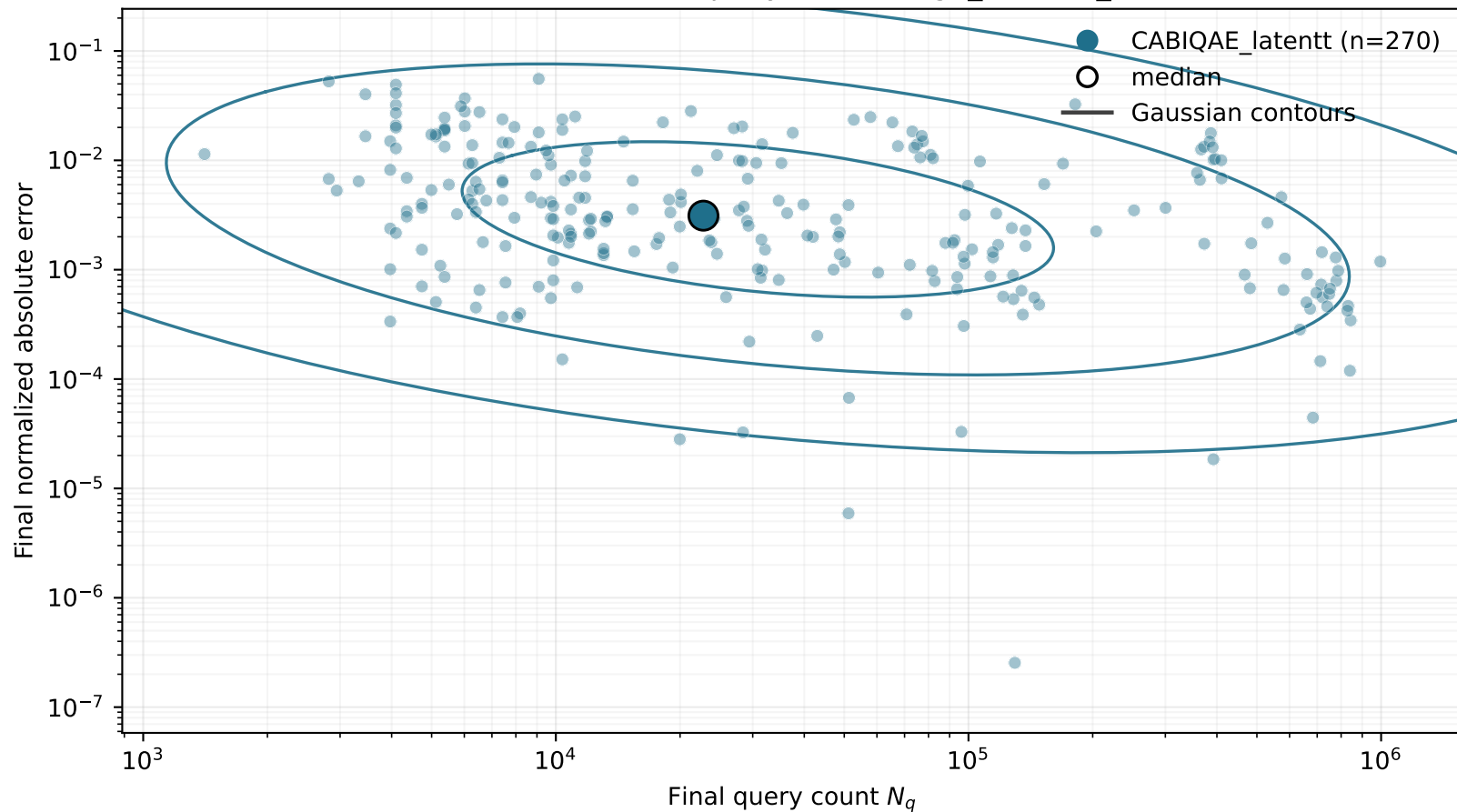
Final error versus query count: large_realistic_v2
