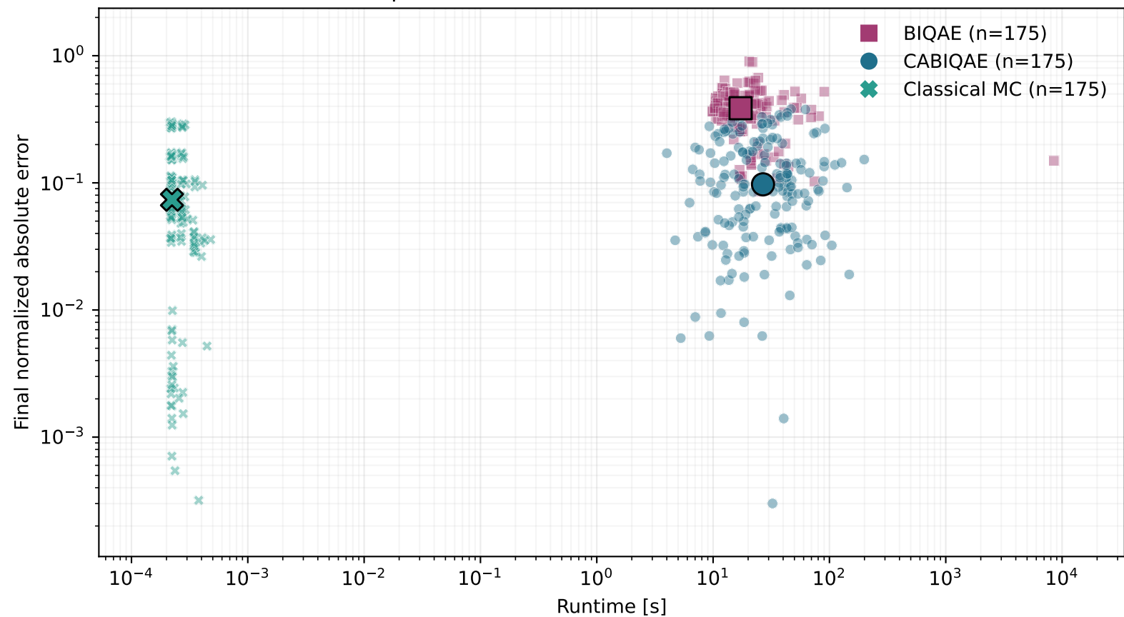
6q CVA AE final CVA error, simulated noise
