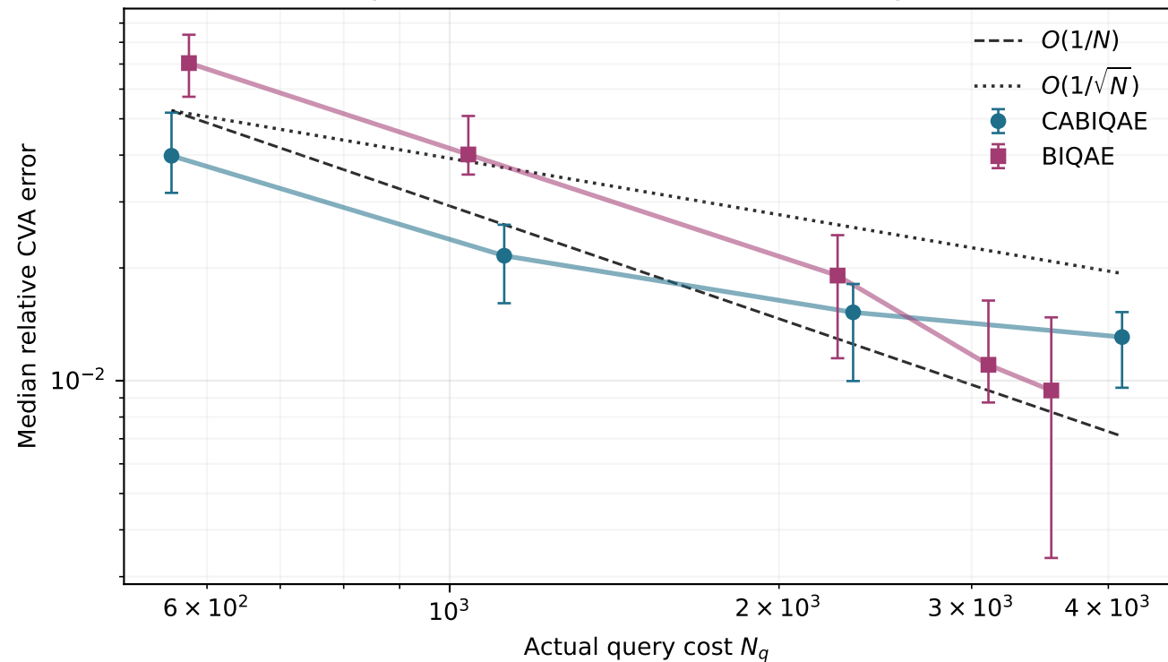
6q CVA AE, simulated noise, fixed budgets
