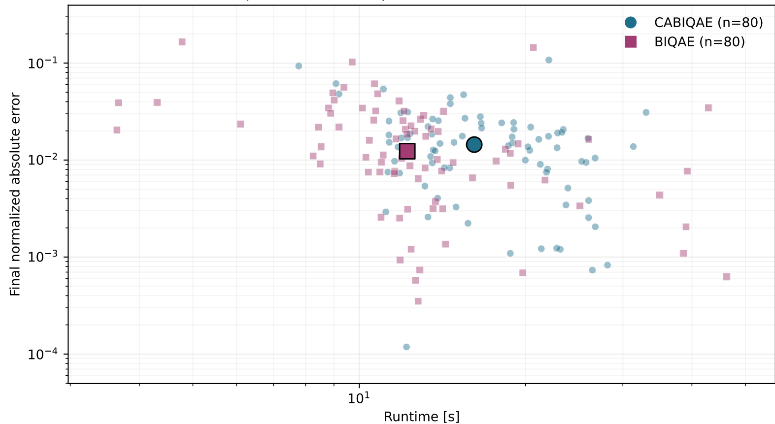
6q CVA AE final amplitude error, simulated noise
