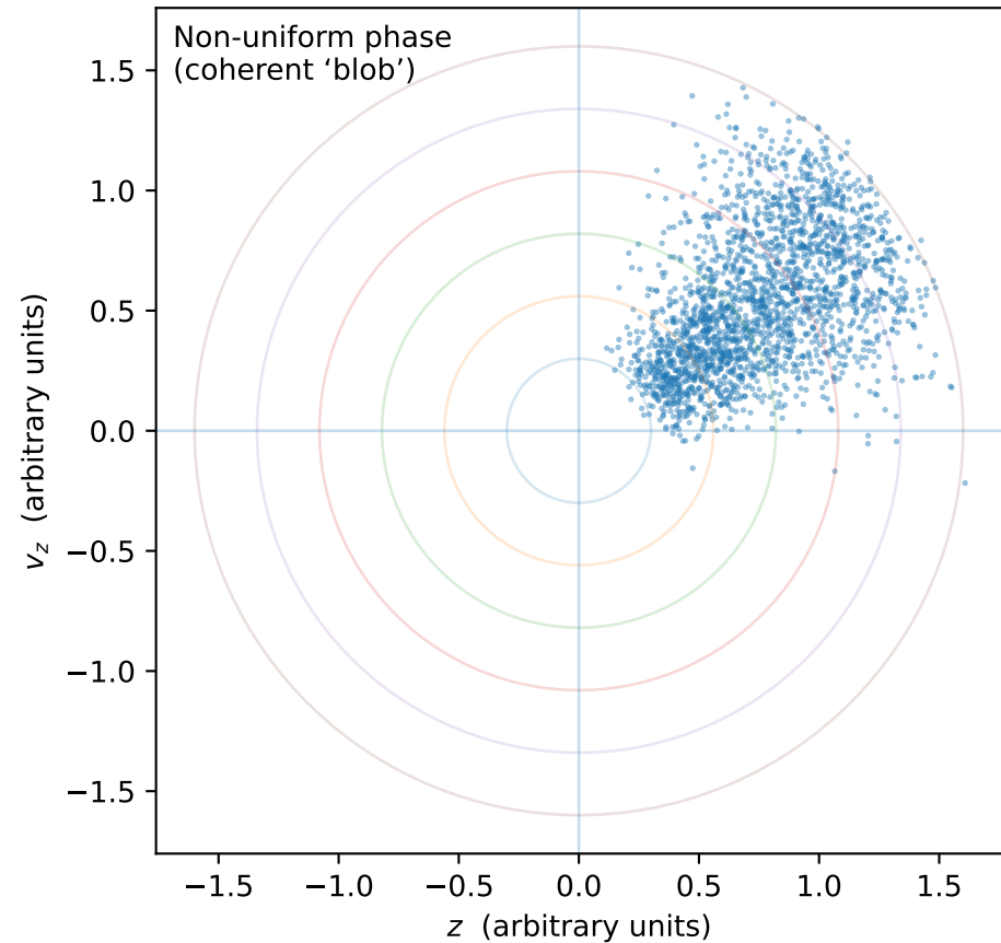
A. Immediately after a vertical perturbation
