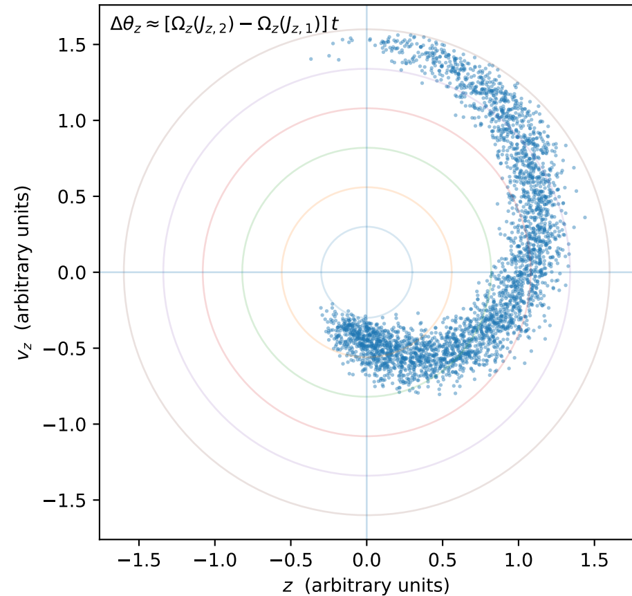
C. Differential winding produces the spiral
