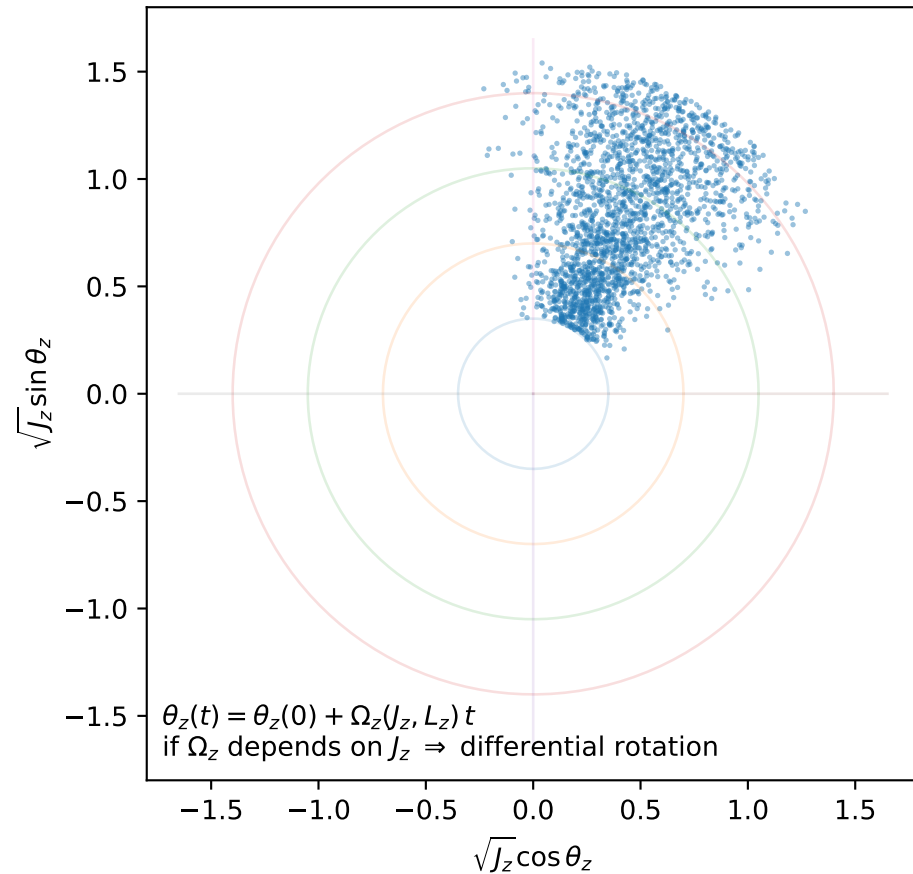
B. In vertical action-angle variables
