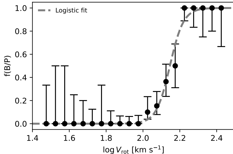
Figure 10 B/P bulges vs rotation velocity
