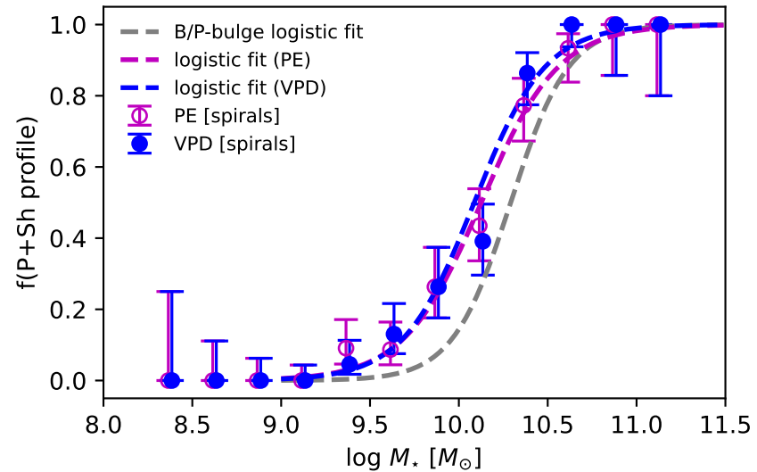
Figure 11 P+Sh profiles vs stellar mass
