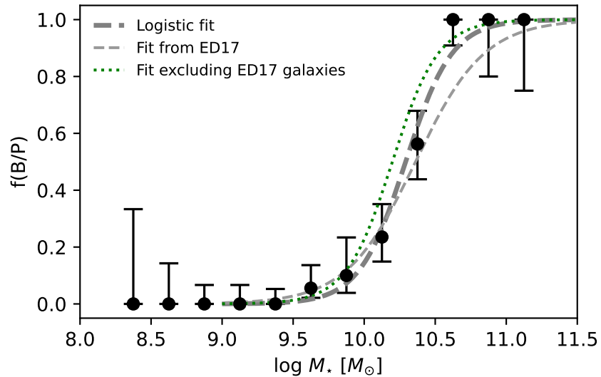
Figure 9 B/P bulges vs stellar mass
