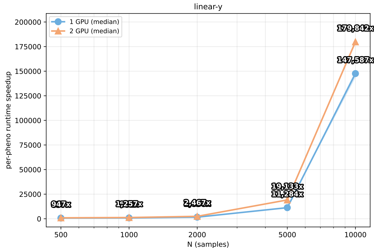
FaSTERLMM vs FaSTLMM speedup (10 parallel jobs, 10 CPU each)
