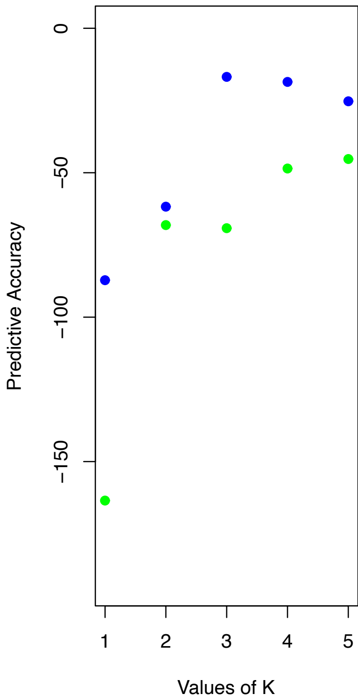
Cross-Validation Results
