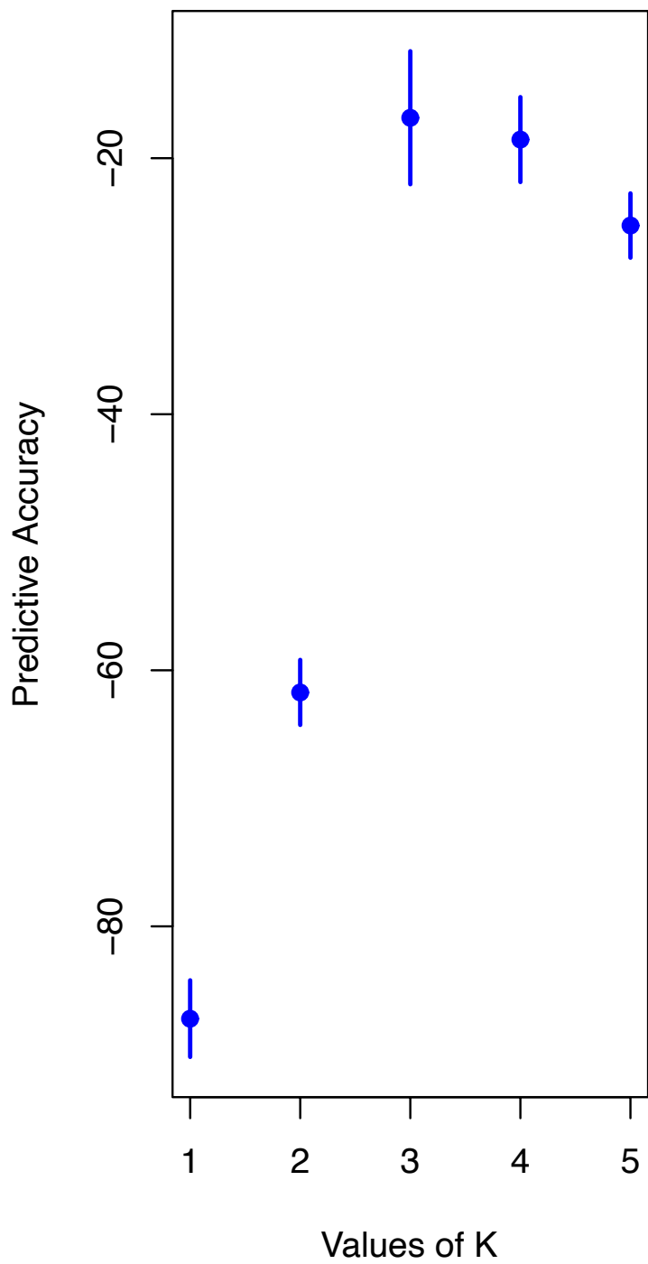
Spatial Cross-Validation Results
