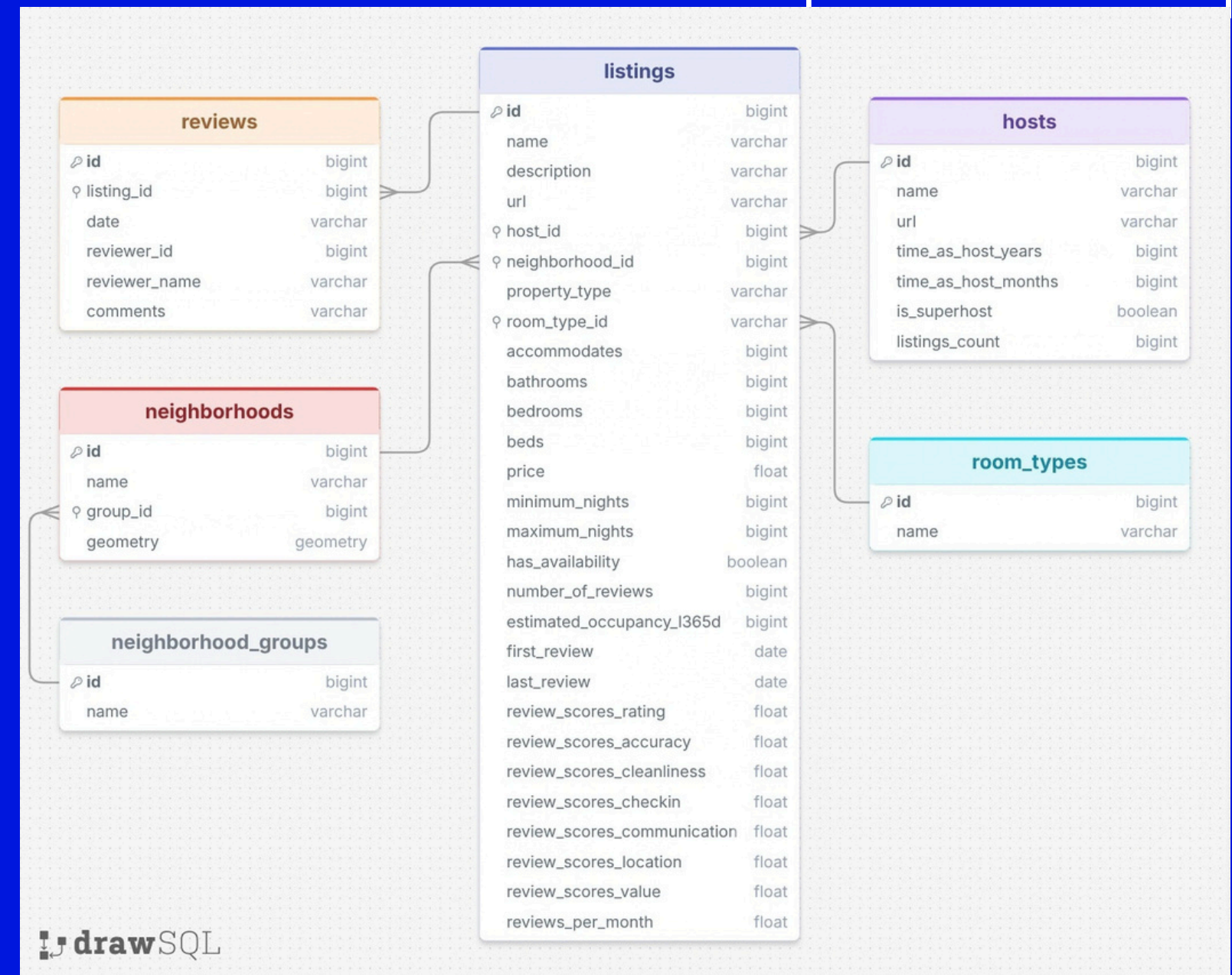
Entity-Relationship Diagram
