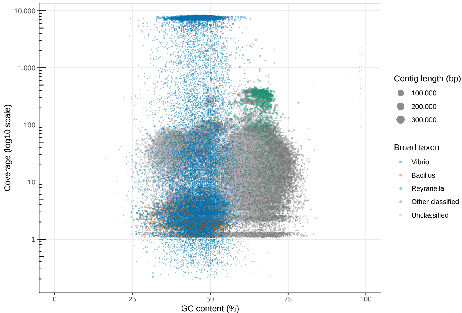
BS0607_9 contigs by GC content and log 10 -scaled coverage
