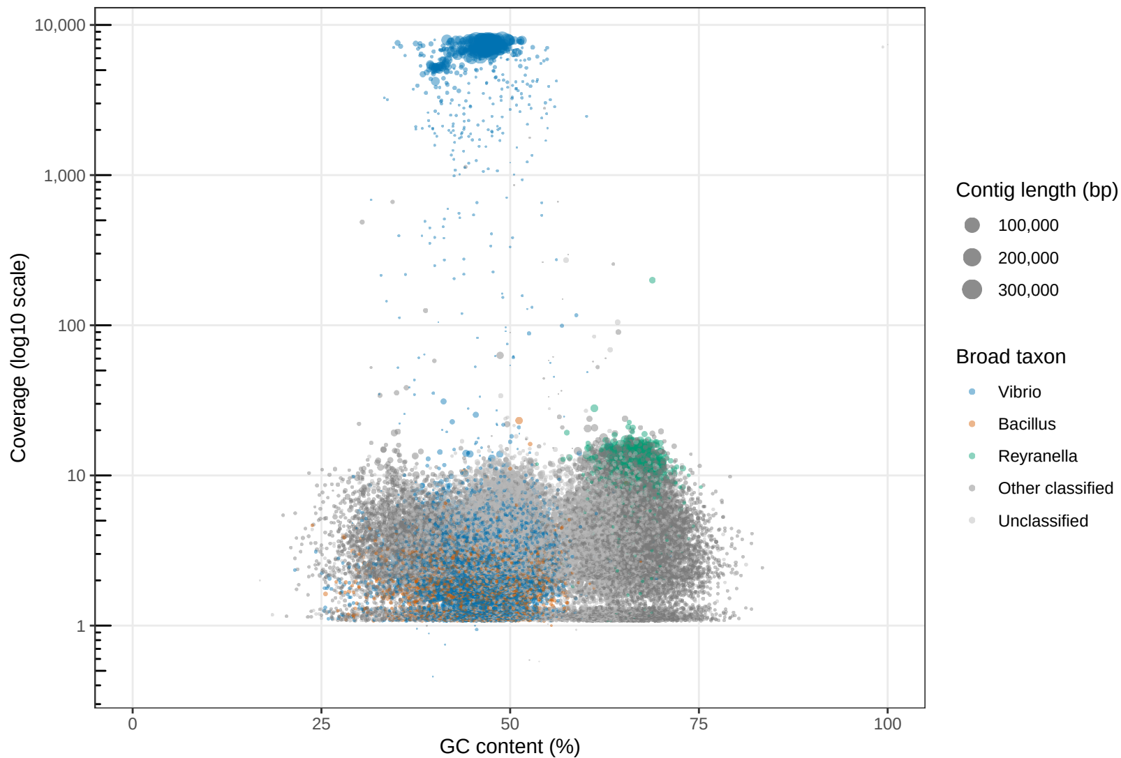
CB0707_82 contigs by GC content and log10-scaled coverage
