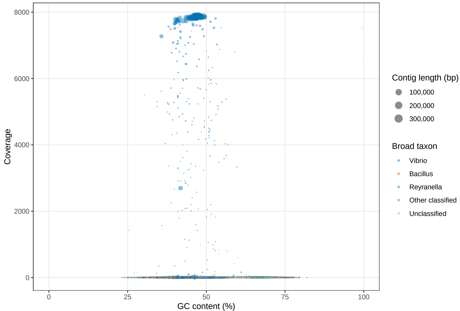
NB0507_8 contigs by GC content and coverage
