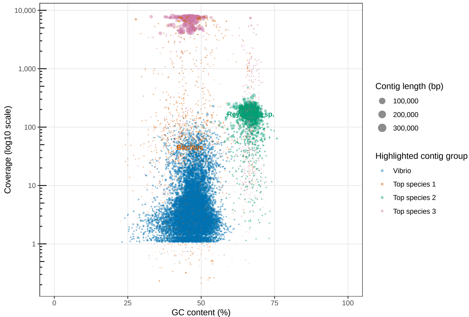
BI0607_2 Vibrio and top species contigs by GC content and log10-scaled coverage
