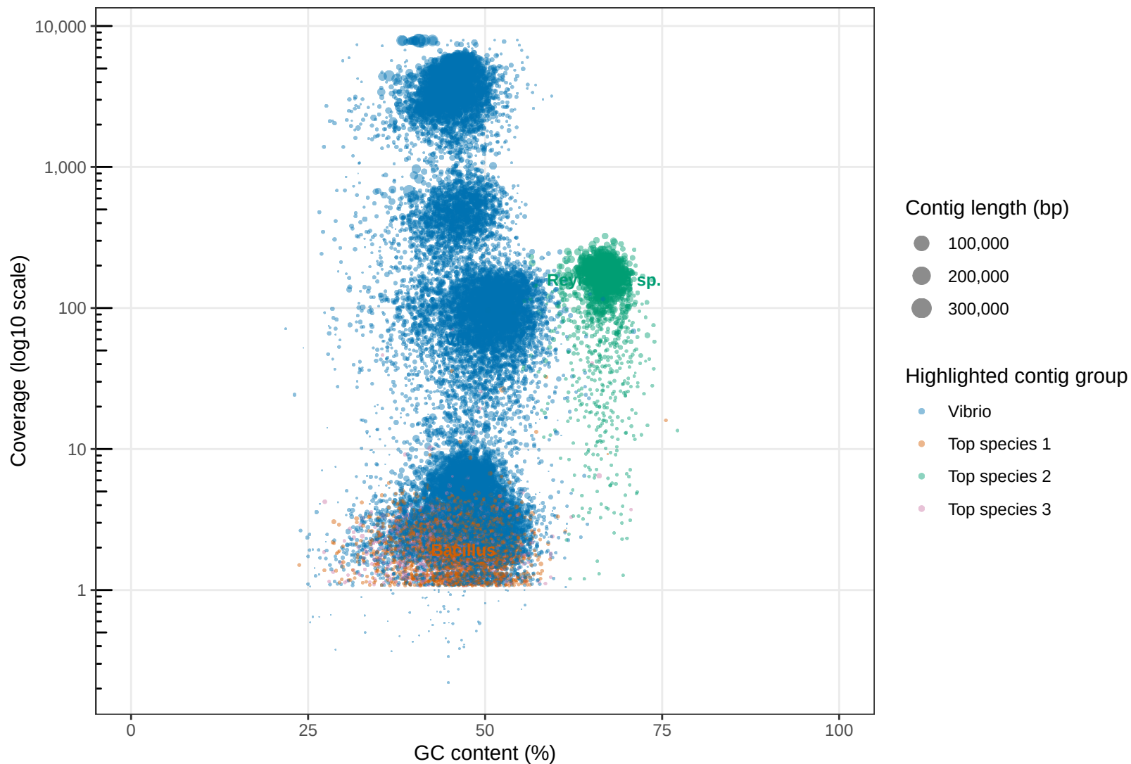
NB0507_14 Vibrio and top species contigs by GC content and log 10 -scaled coverage
