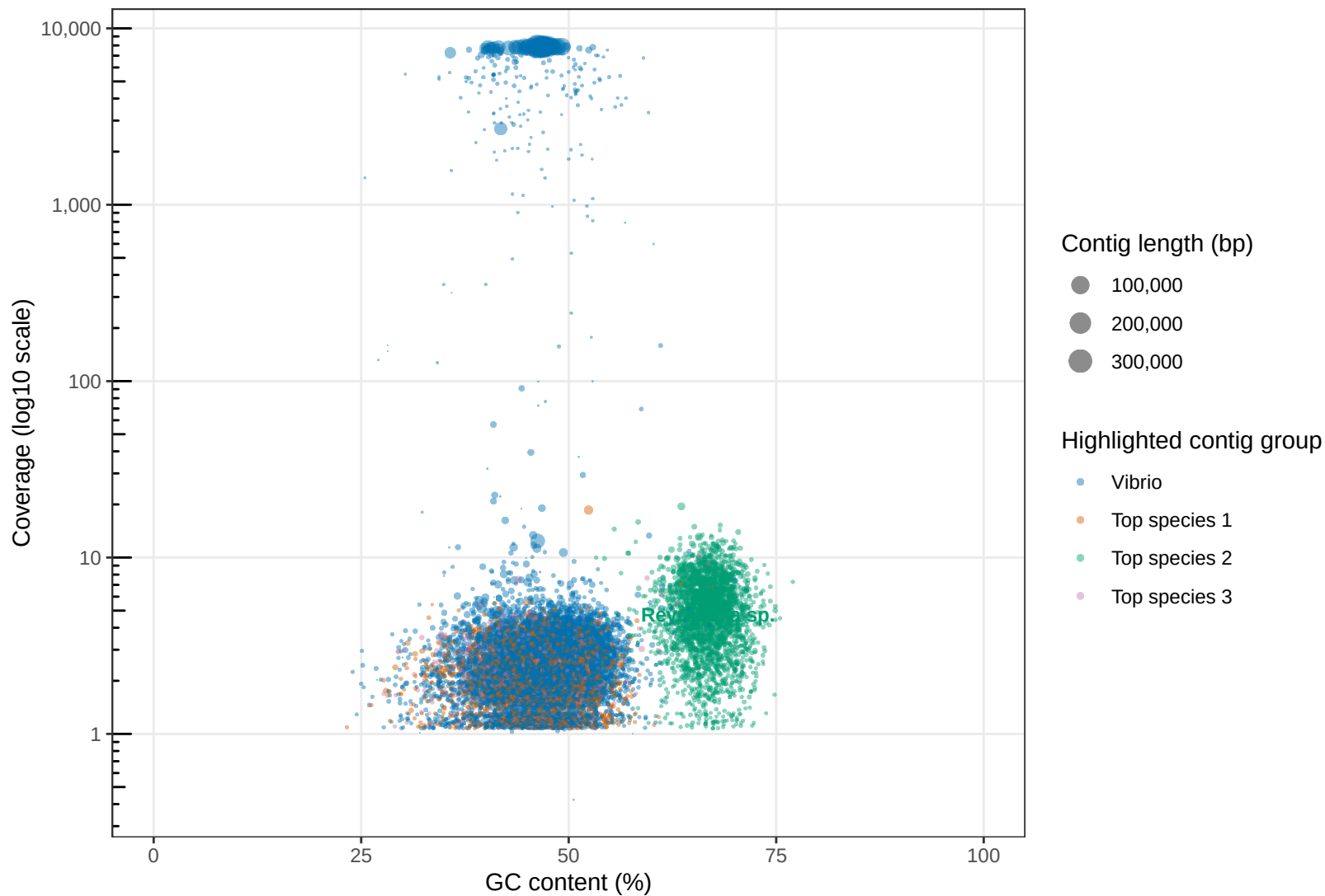
NB0507_8 Vibrio and top species contigs by GC content and log10-scaled coverage
