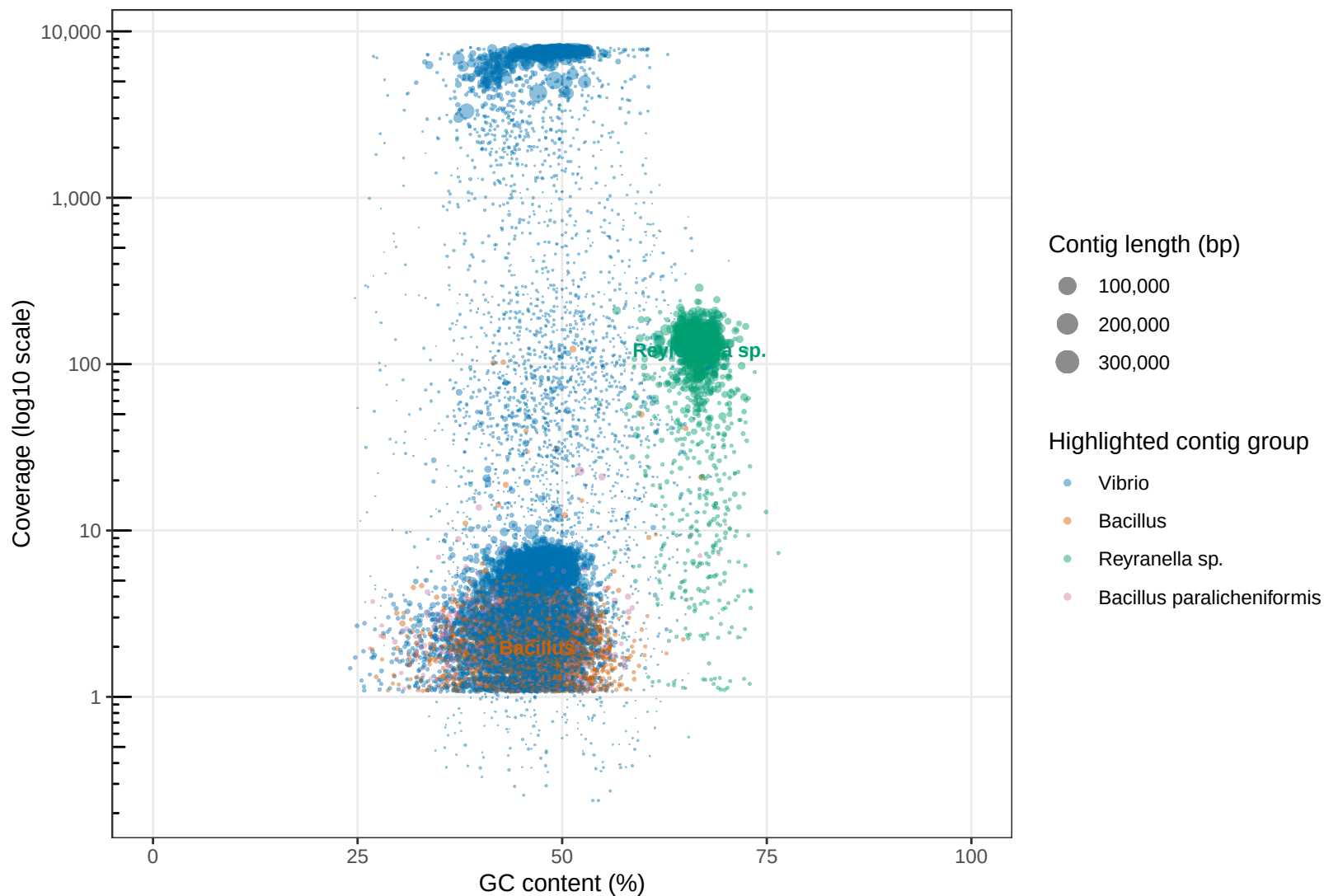
BI0607_1 Vibrio and top species contigs by GC content and log10-scaled coverage
