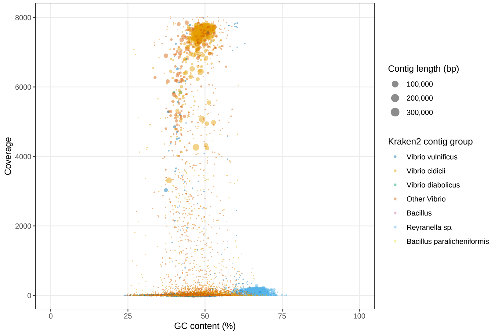
BI0607_1 top Vibrio and other species contigs by GC content and coverage
