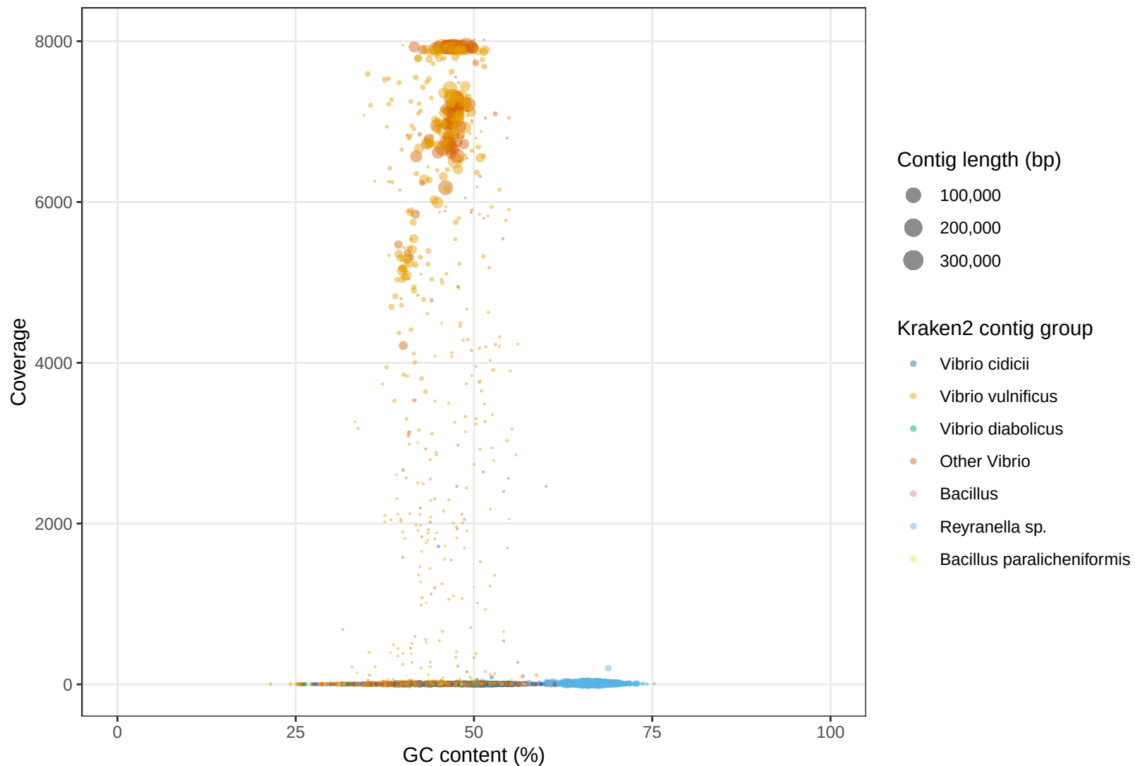
CB0707_82 top Vibrio and other species contigs by GC content and coverage
