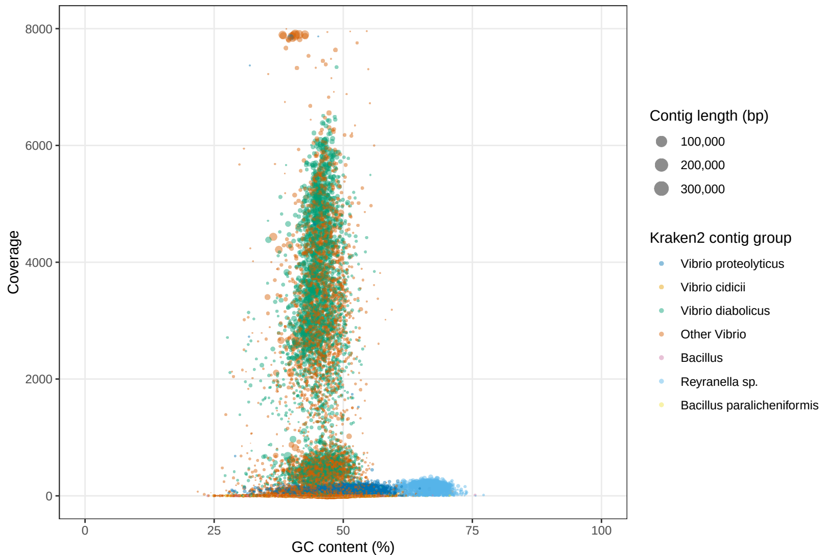
NB0507_14 top Vibrio and other species contigs by GC content and coverage
