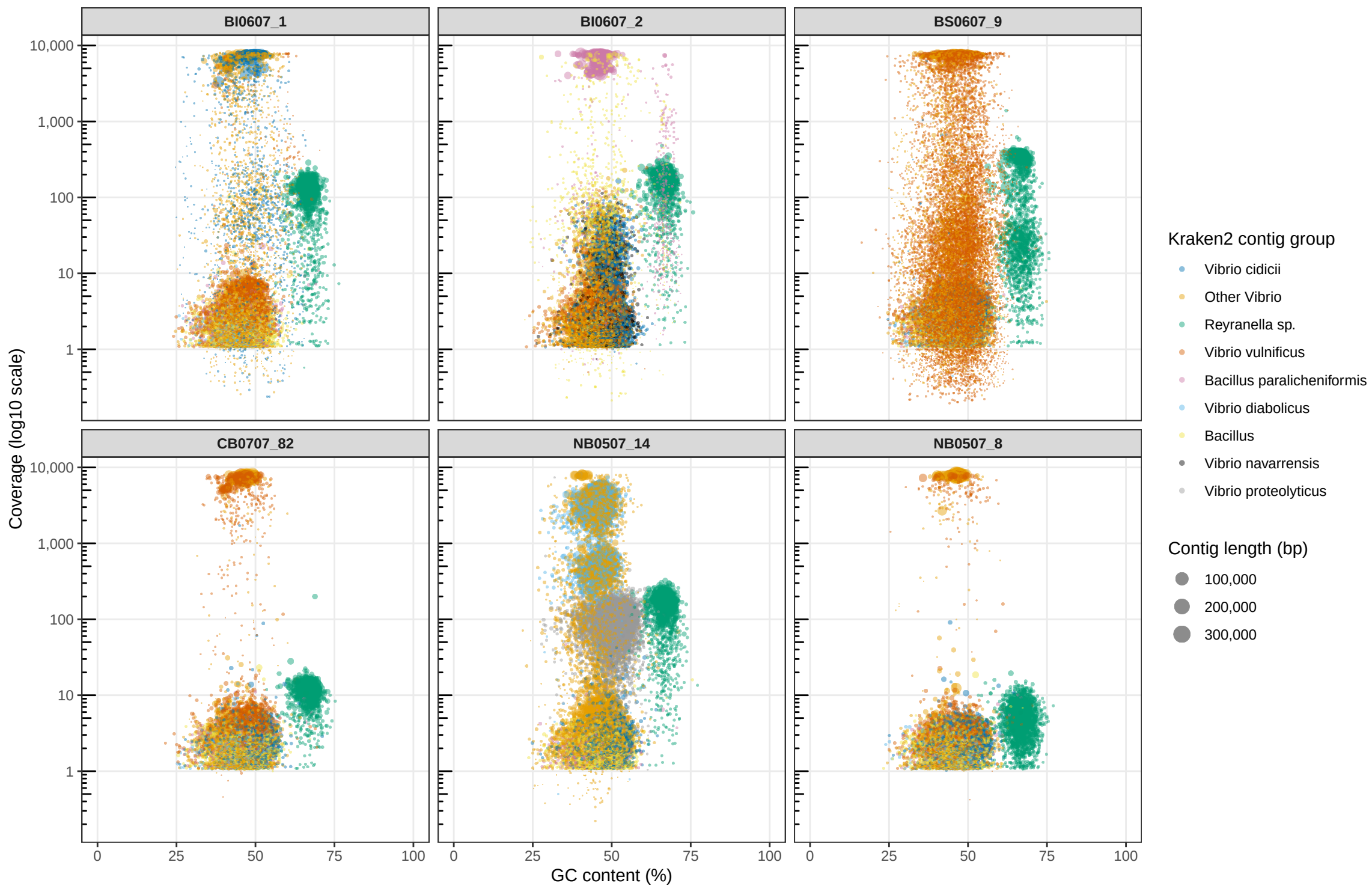
Six-sample contig GC content and log10-scaled coverage
