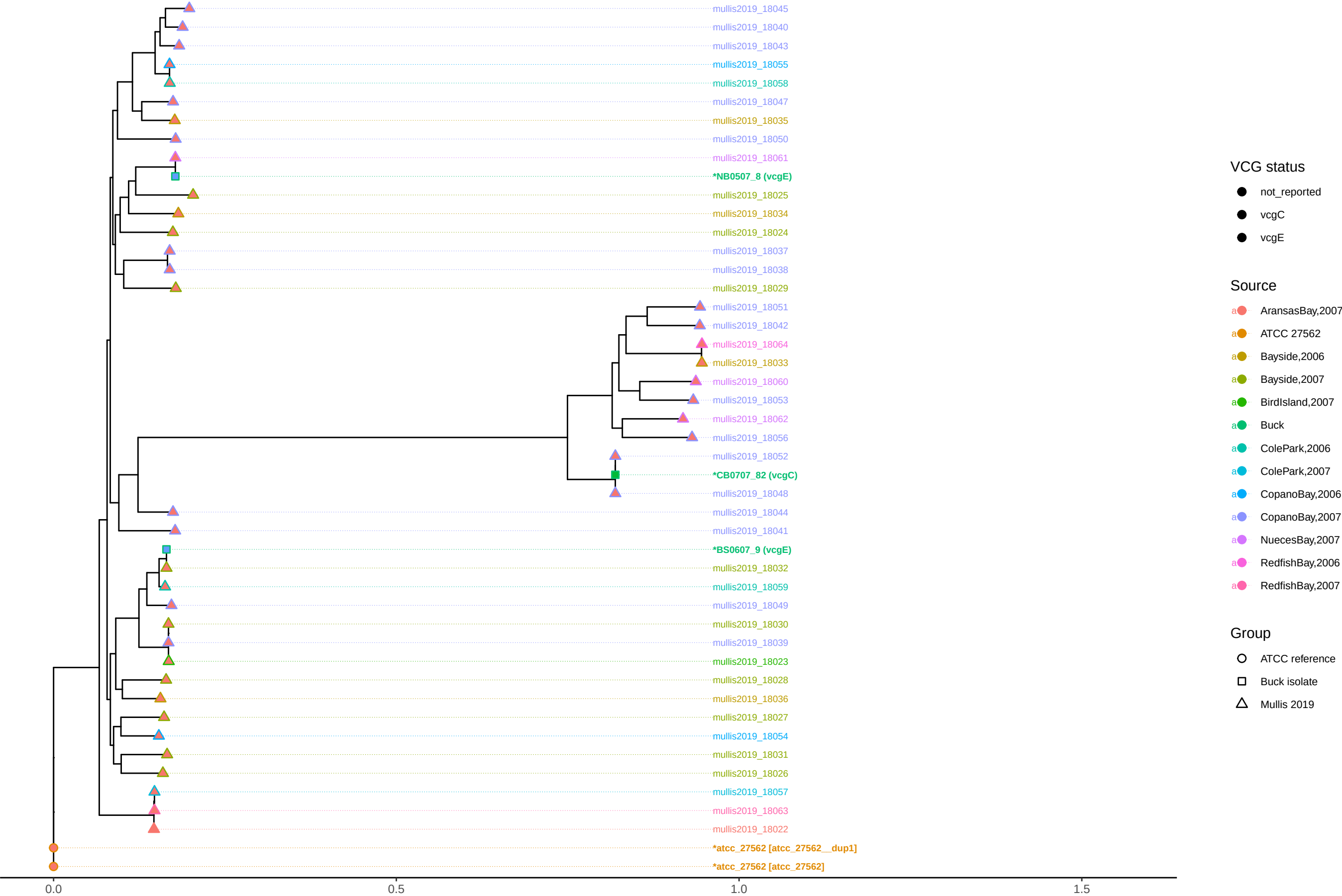
Expanded V. vulnificus 46-genome RAxML-NG support tree
