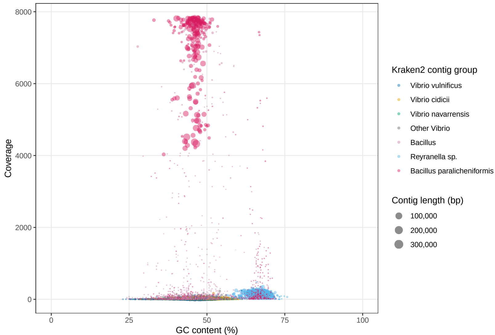
BI0607_2 top Vibrio and other species contigs by GC content and coverage
