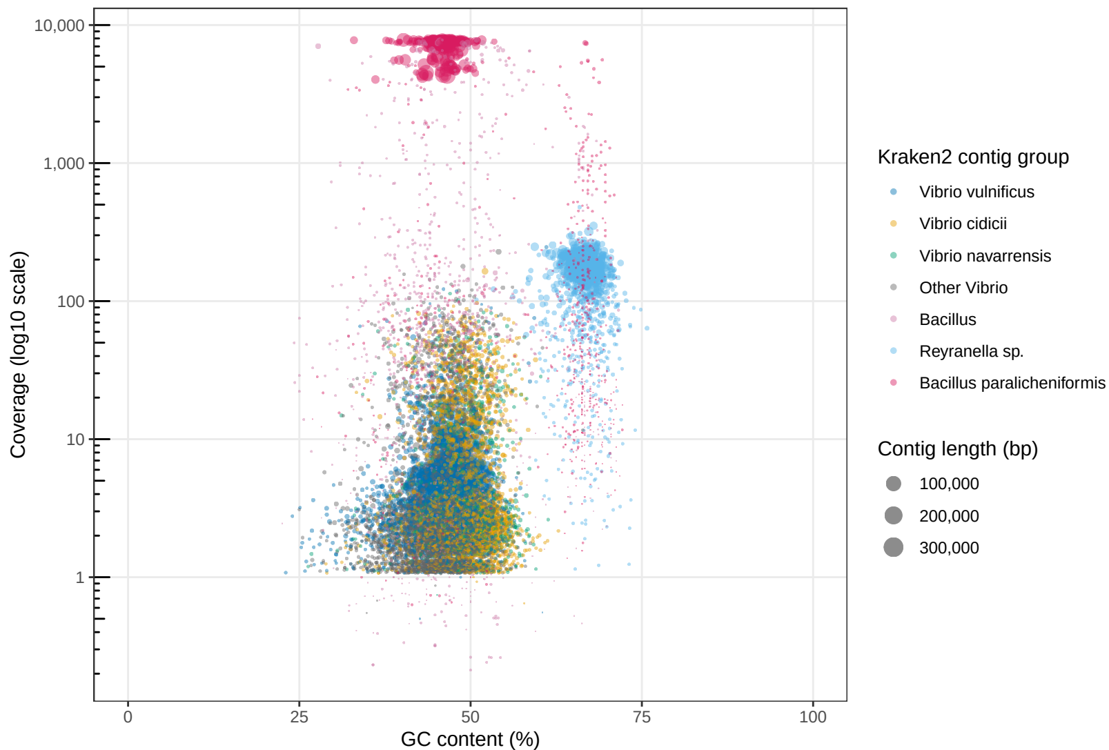
BI0607_2 top Vibrio and other species contigs by GC content and log 10 -scaled coverage
