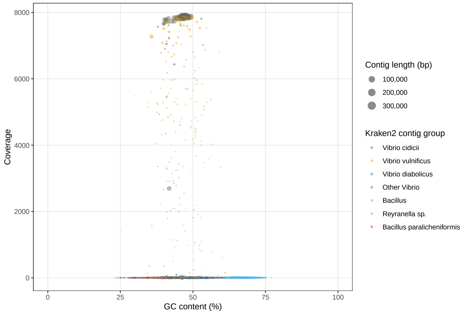
NB0507_8 top Vibrio and other species contigs by GC content and coverage
