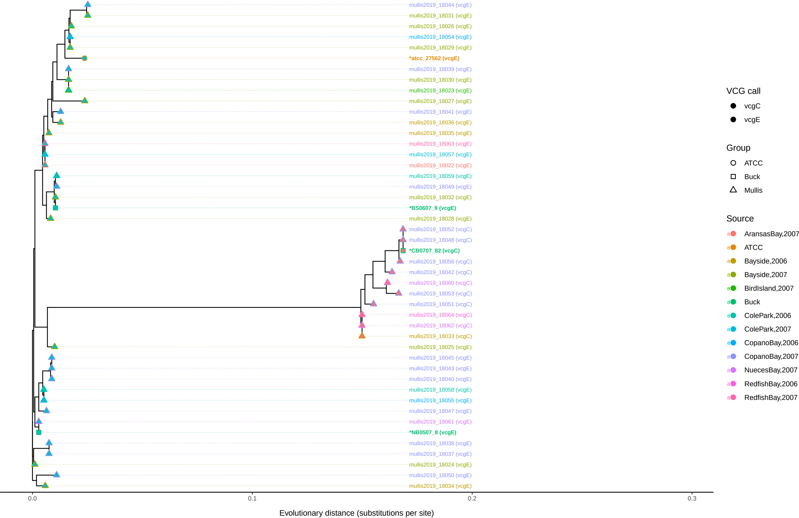
Expanded V. vulnificus 46-genome vcg-marker FastTree
