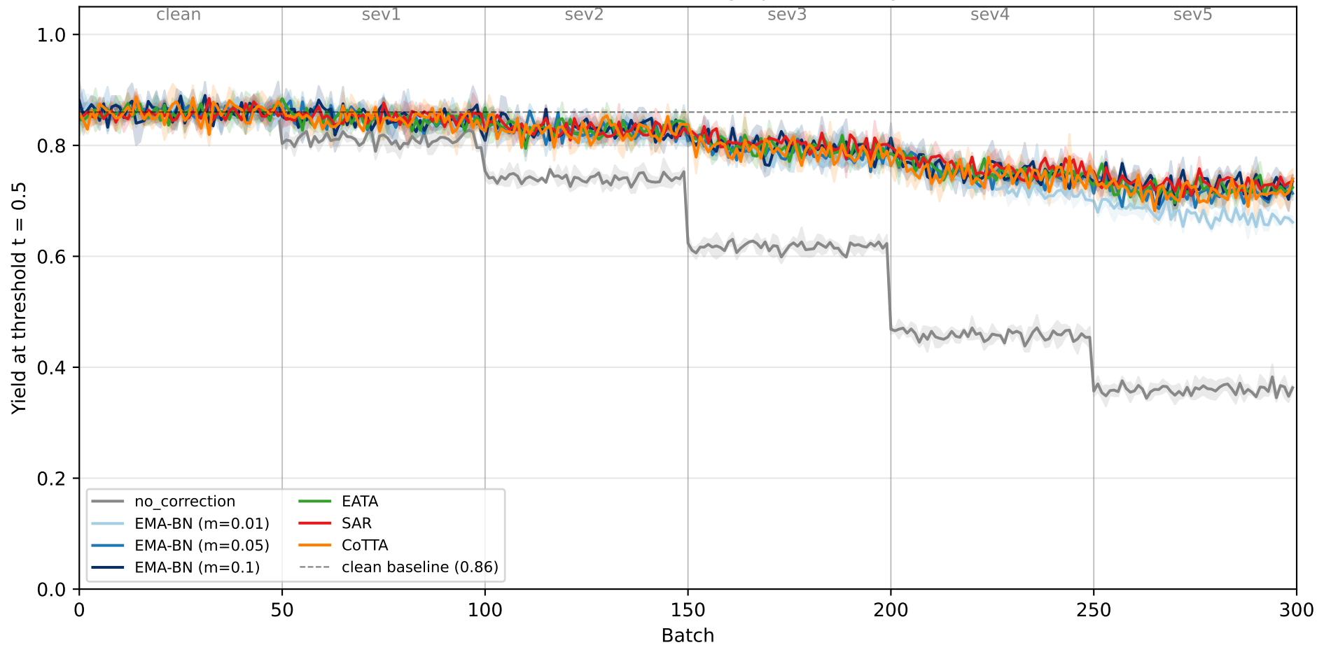
RQ1: yield trajectories under gradual degradation — blur (MOCK DATA — for design preview only)
