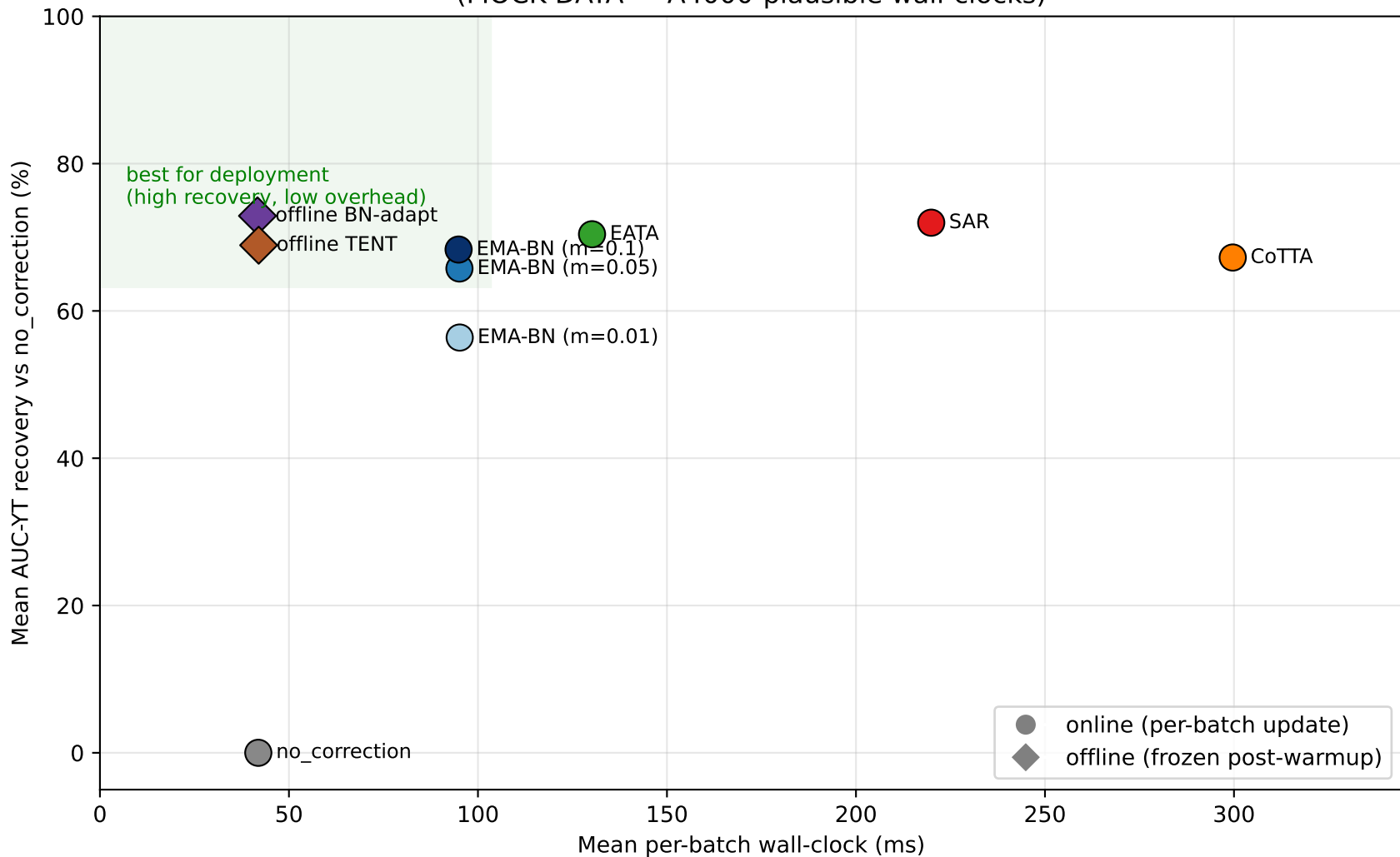
RQ4: efficiency vs recovery — averaged over all corruptions × scenarios (MOCK DATA — A4000-plausible wall-clocks)
