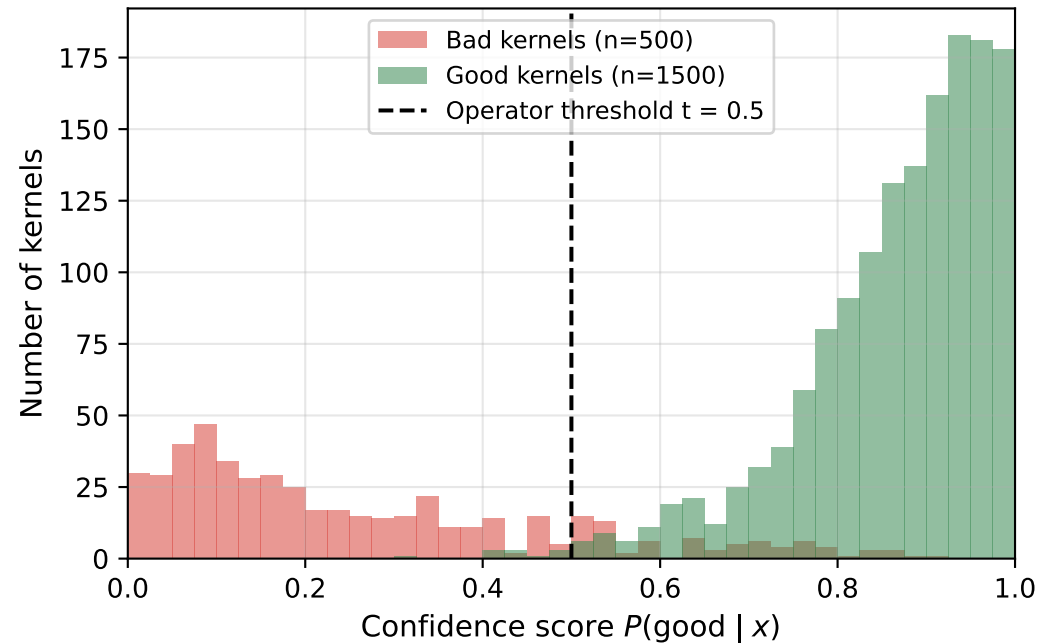
(a) Distribution of confidence scores
