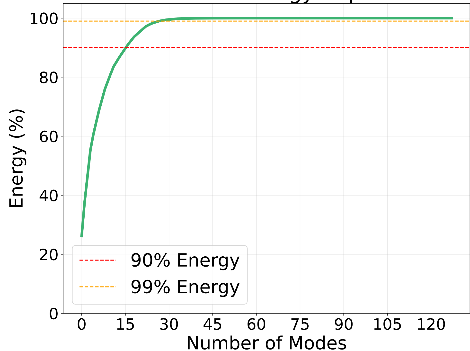
Cumulative Energy Captured
