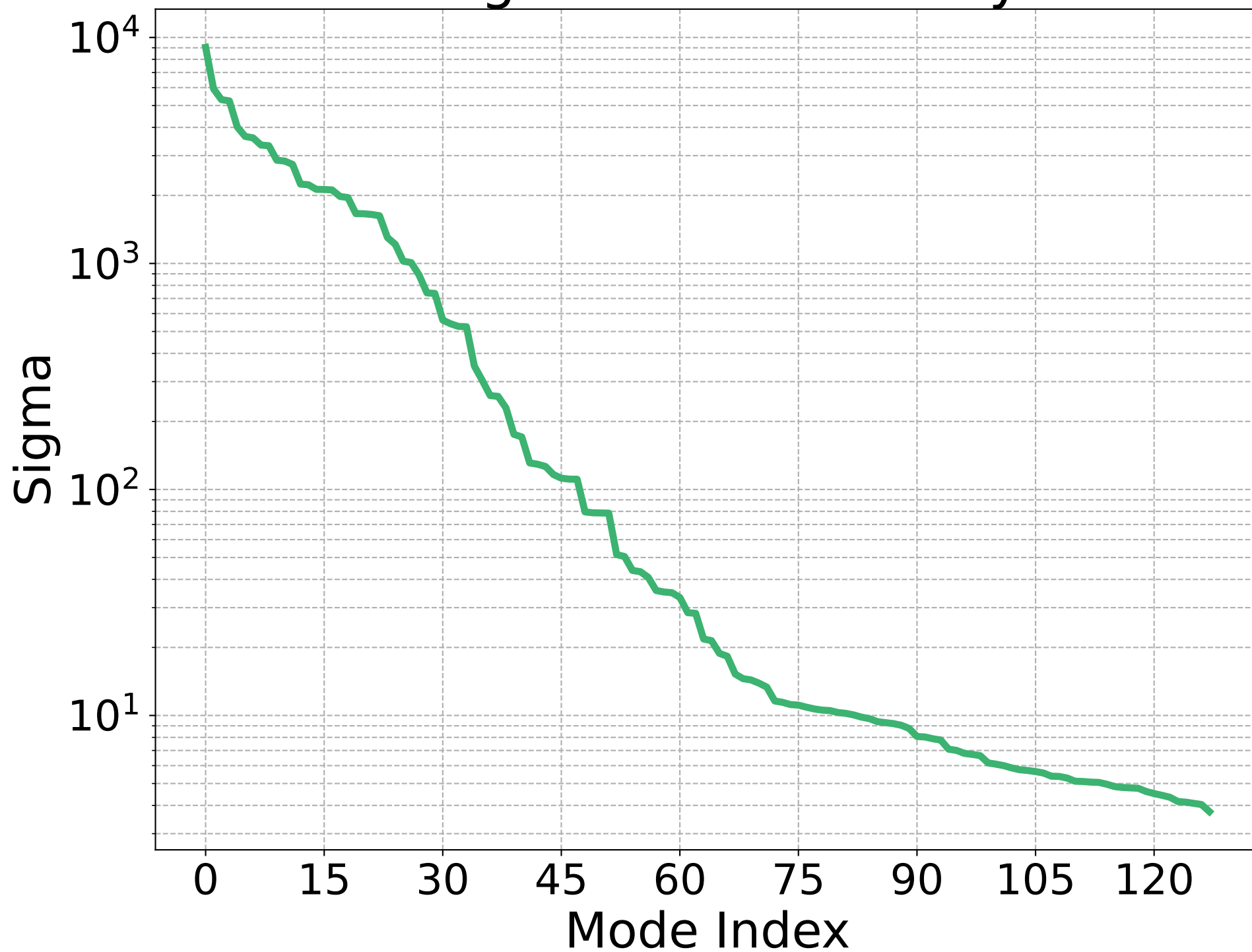
Singular Values Decay
