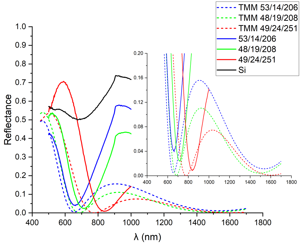
Figure 4.13: Reflectivities of antireflective coatings with varying layer thicknesses simulated using the transfer matrix method and measured experimentally. The reflectance of a bare Si wafer is included for comparison.
