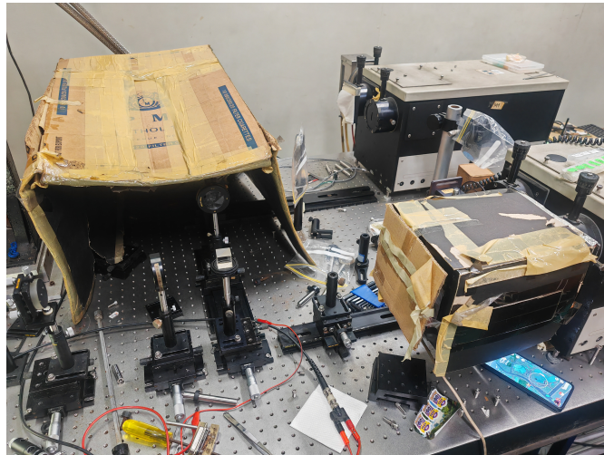
Figure 3.1: Normal incidence reflectance spectroscopy setup.
