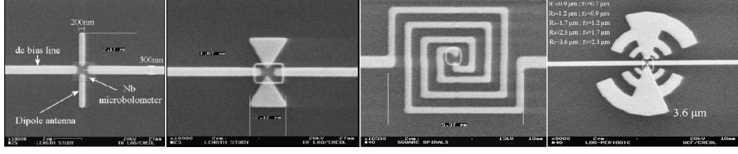
Figure 2.2: Commonly used THz PCA geometries; from left to right: dipole, bowtie, spiral, and log-spiral[16]
