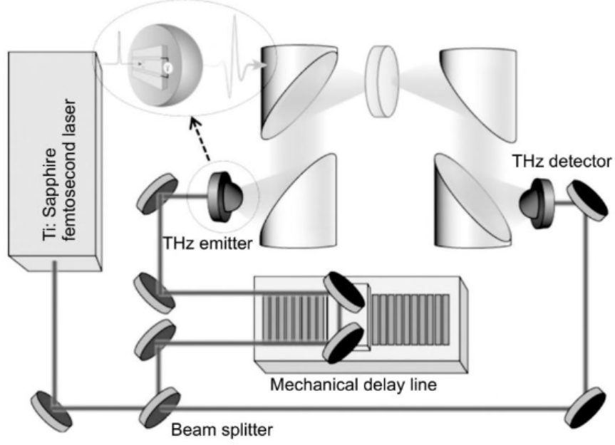
Figure 2.3: Schematic of a THz TDS setup with a femtosecond laser and two photoconductive antennas[7]
