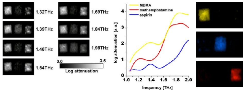
Figure 2.1: THz identification of MDMA, methamphetamine, and aspirin through a paper envelope. The substances are differentiated using their THz spectra[13]
