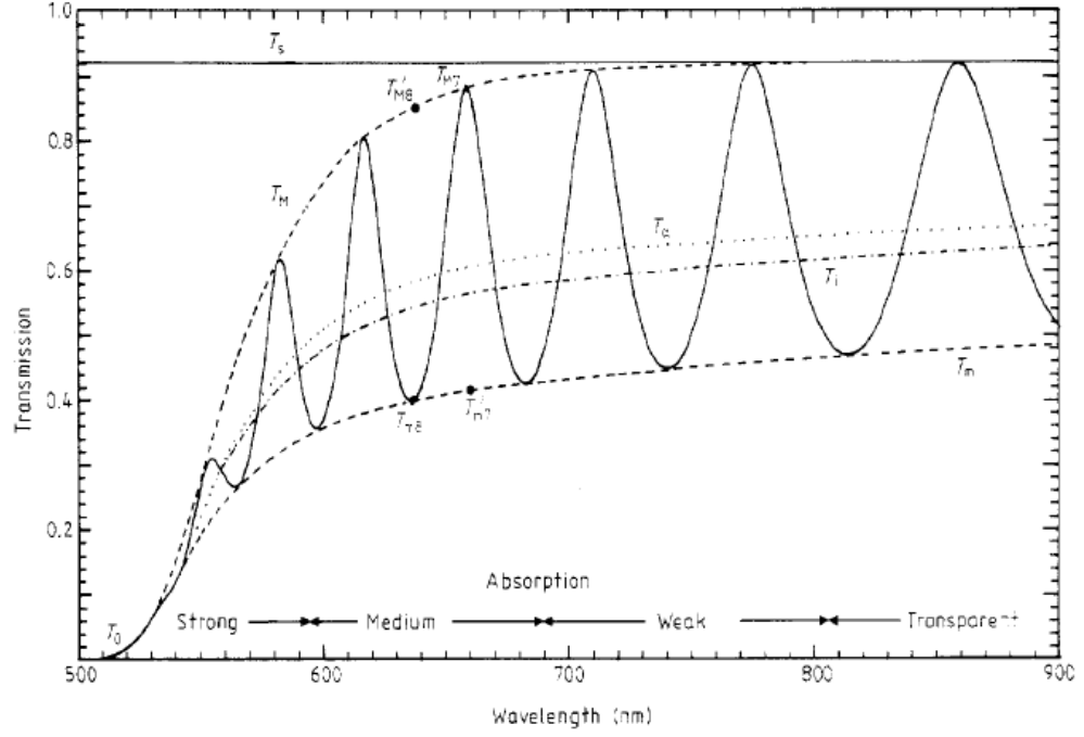
Figure 2.8: Envelope method as described by Swanepoel for a 1 \mu\text{m} film of a-Si:H on a finite glass substrate with transmittance T_s .
