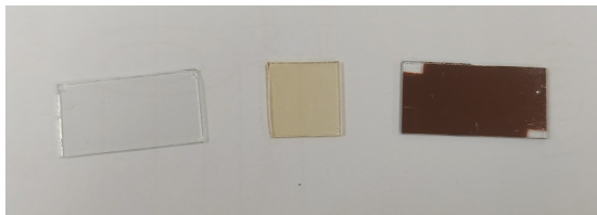
Figure 4.1: Bare glass, 0.138 kÅ and 3.050 kÅ thick a-Si films on glass. The intensity of the tint increases with the deposited a-Si thickness due to the absorption of Si in the visible range.
