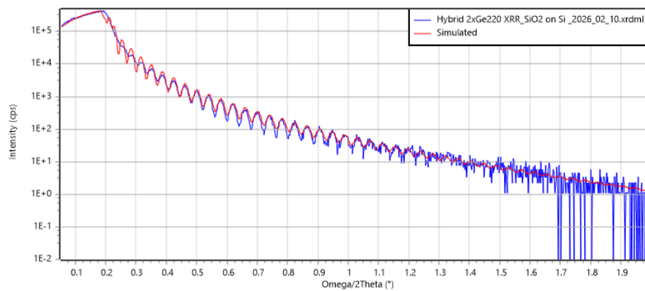
Figure 4.9: XRR curve fit to 103.9 nm \text{SiO}_2 thin film
