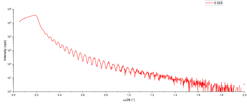
(a) 0.525 kÅ SiO 2 thin film
