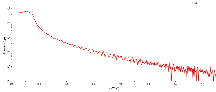
(b) 0.884 kÅ SiO 2 thin film
