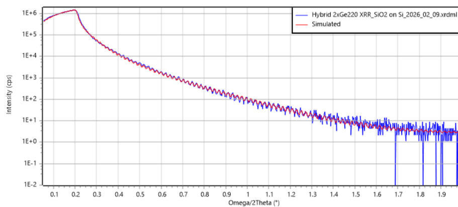
Figure 4.10: XRR curve fit to 204.7 nm \text{SiO}_2 thin film
