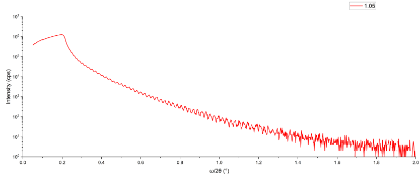
(c) 1.050 kÅ SiO 2 thin film
